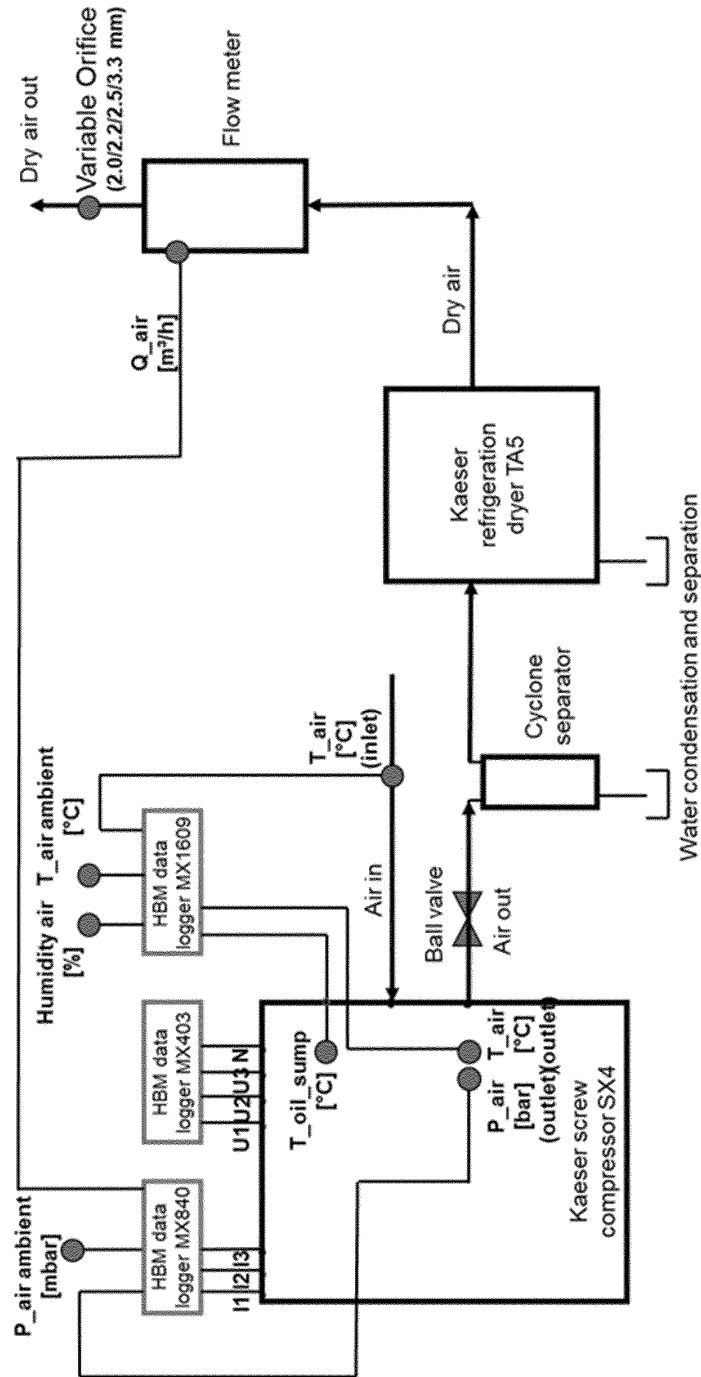
Figure 1: Illustration of the test settings used to determine the effects on energy consumption in an air compressor.
