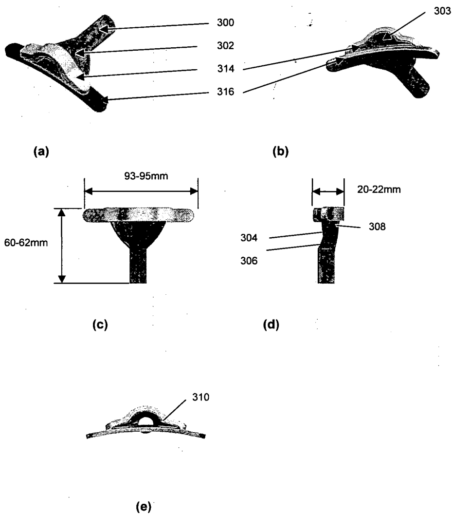
Figure 4: Nozzle design without clip
