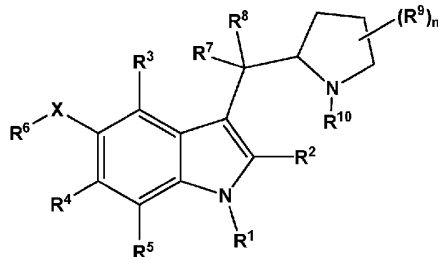
Formula (I)
