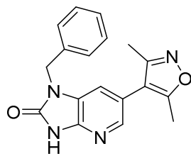
Compound E:
