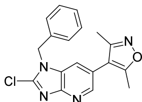
Compound F:
