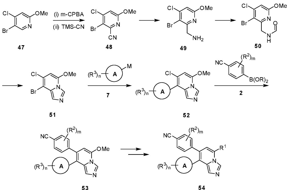
Scheme 8
