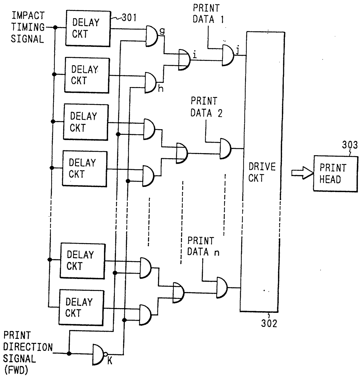
FIG. 18 PRIOR ART
