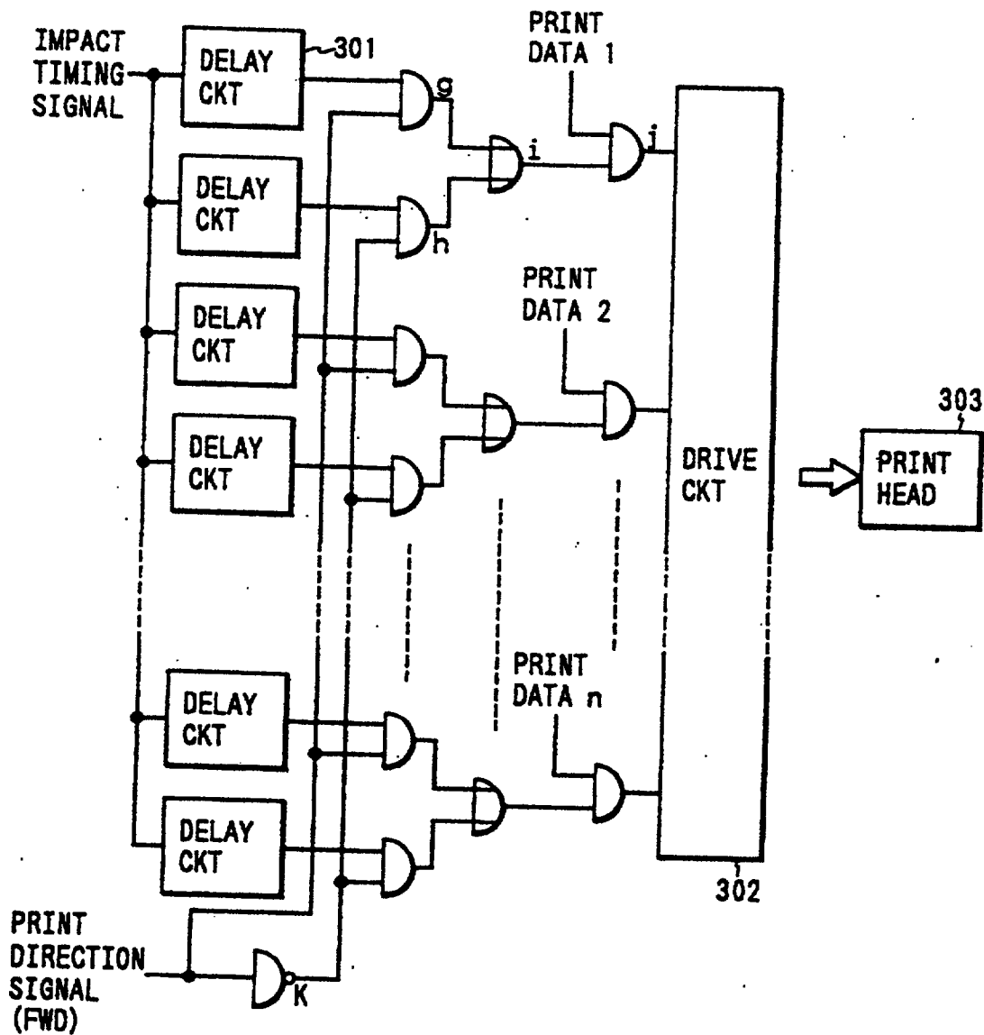
FIG. 18 PRIOR ART
