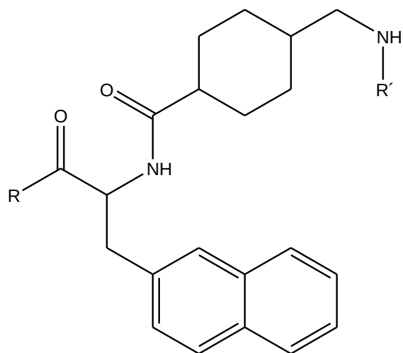
(2-Nal)-(Chx)
