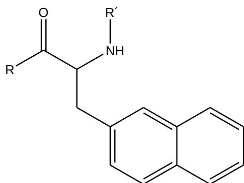
(2-Nal)
