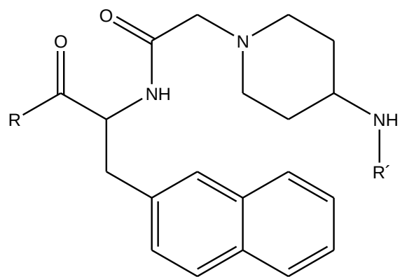
(2-Nal)-(AcAP)
