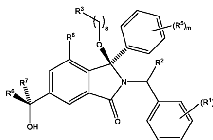
Diastereoisomer 2B
