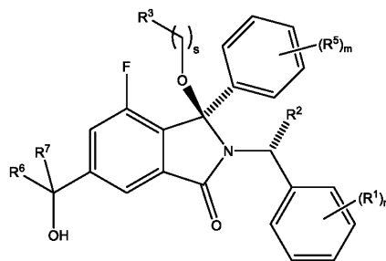
Diastereoisomer 1B
