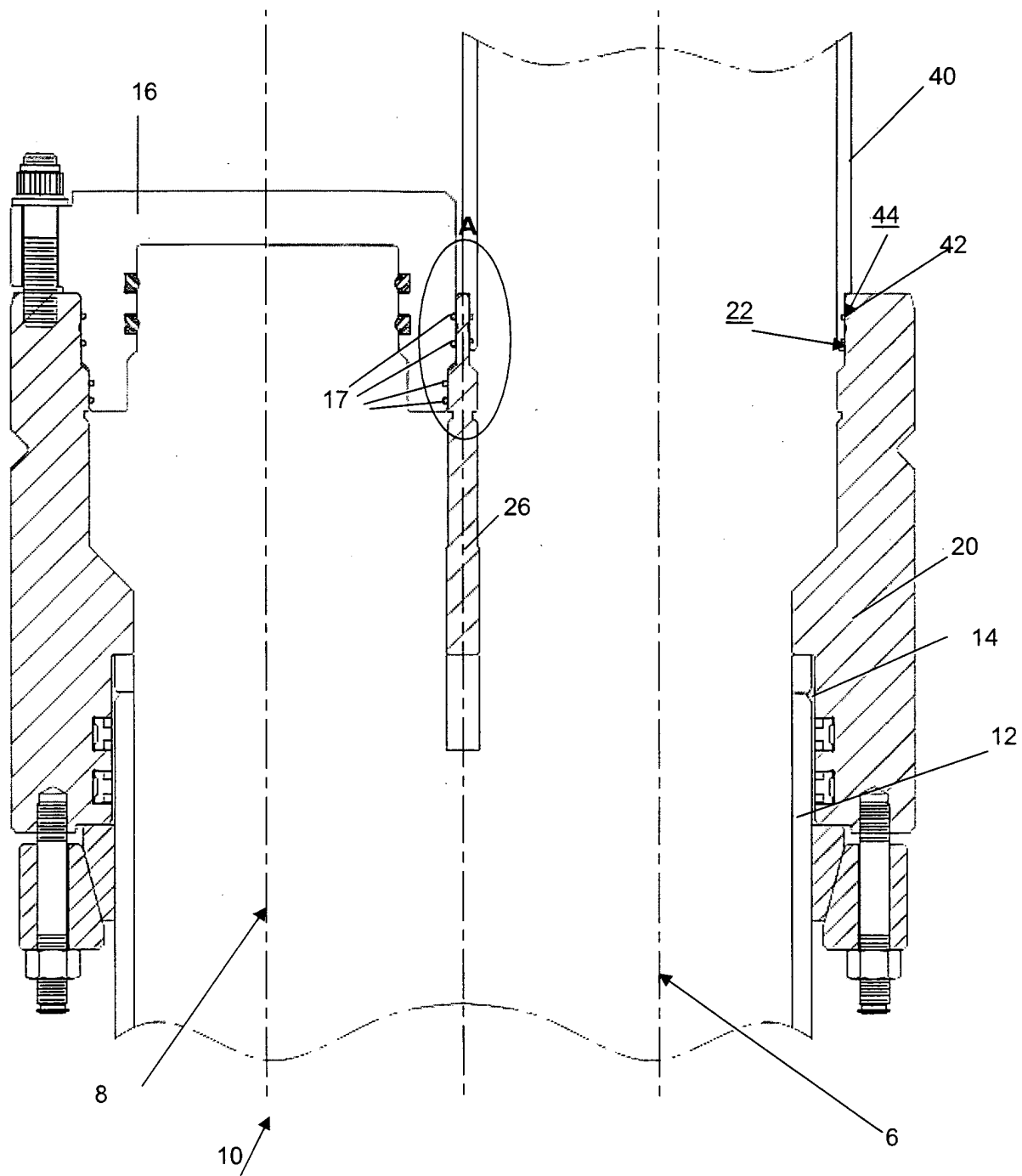
Figure 1 (PRIOR ART)
