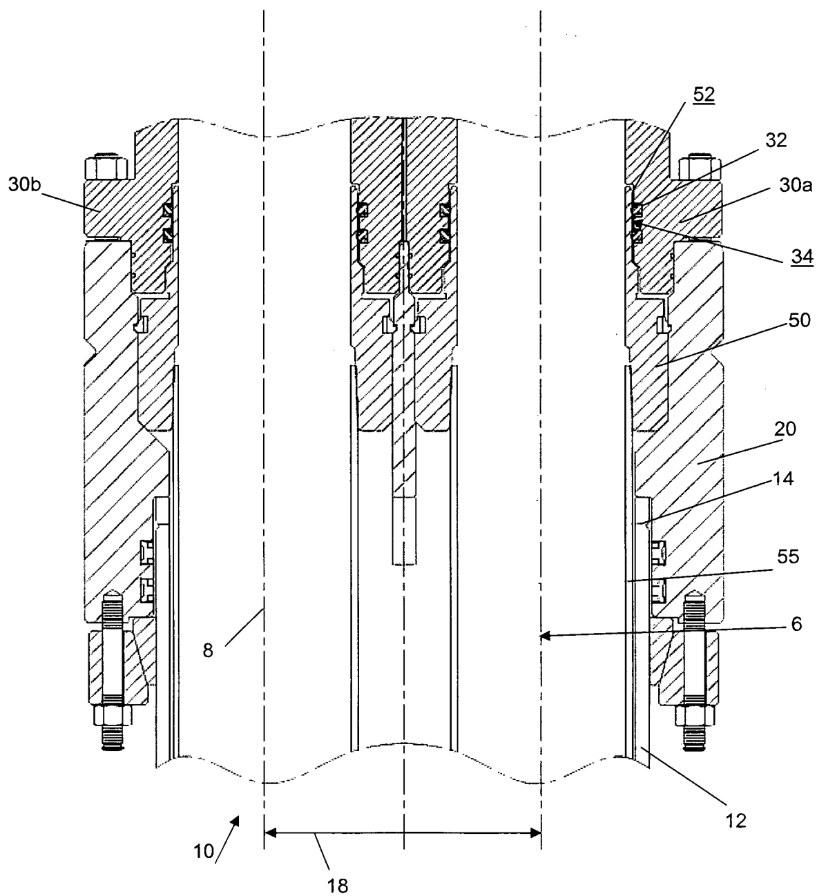
Figure 2 (PRIOR ART)
