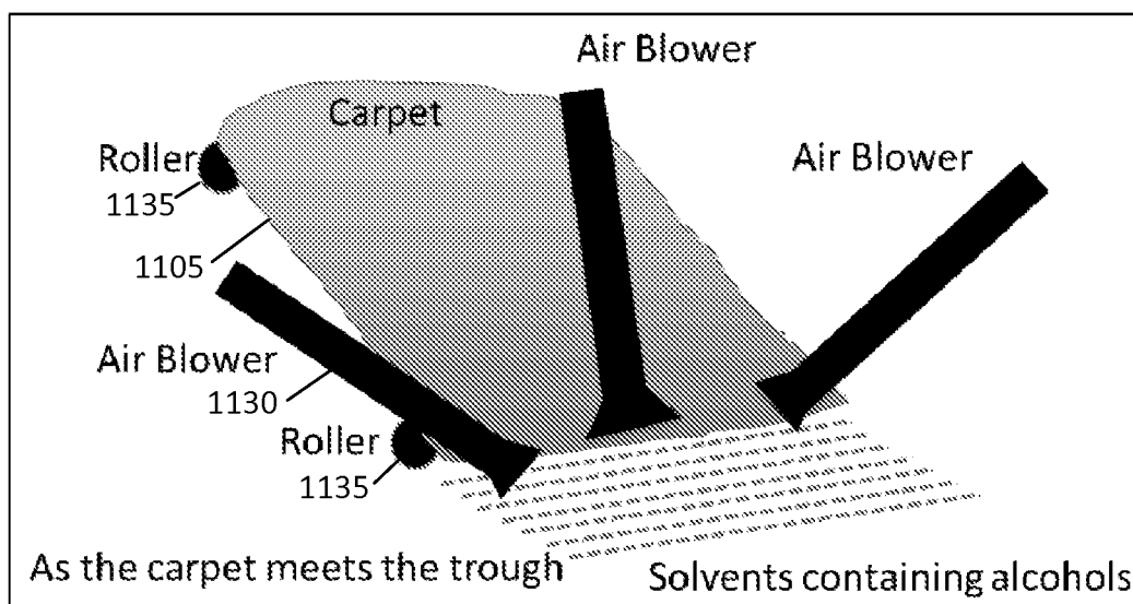
(b) Solution Treatment System (front view)
