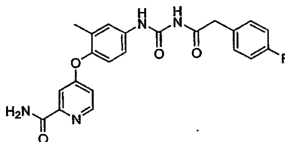
1-(4-(2-Carbamoylpyridin-4-yloxy)-3-methylphenyl)-3-(2-(4-fluorophenyl)acetyl)urea
