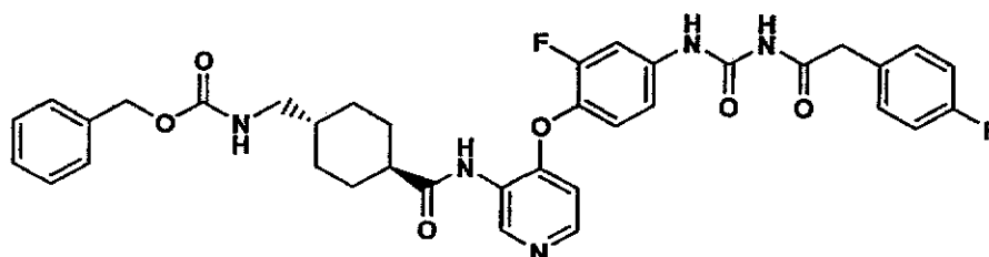
1-(4-(3-((1R,4R)-4-(Aminomethyl)cyclohexanecarboxamido)pyridin-4-yloxy)-3-fluorophenyl)-3-(2-(4-fluorophenyl)acetyl)urea
