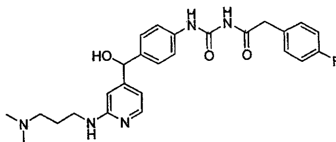
1-(4-((2-(3-(Dimethylamino)propylamino)pyridin-4-yl)(hydroxy)methyl)phenyl)-3-(2-(4-fluorophenyl)acetyl)urea
