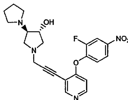
A) (3R,4R)-1-(3-(4-(2-Fluoro-4-nitrophenoxy)pyridin-3-yl)prop-2-yn-1-yl)-4-(pyrrolidin-1-yl)pyrrolidin-3-ol
