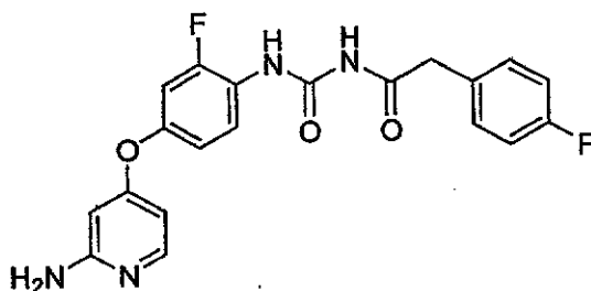
1-(4-(2-Aminopyridin-4-yloxy)-2-fluorophenyl)-3-(2-(4-fluorophenyl)acetyl)urea, trifluoroacetic acid salt
