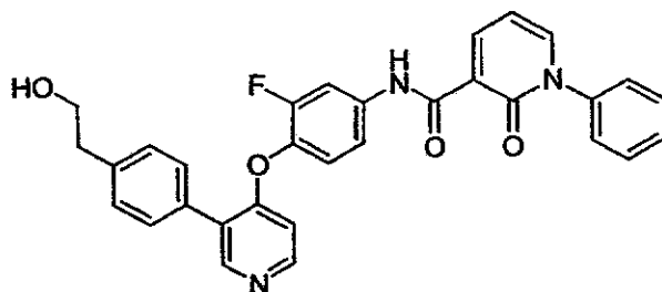
N -(3-Fluoro-4-(3-(4-(2-hydroxyethyl)phenyl)pyridin-4-yloxy)phenyl)-2-oxo-1-phenyl-1,2-dihydropyridine-3-carboxamide
