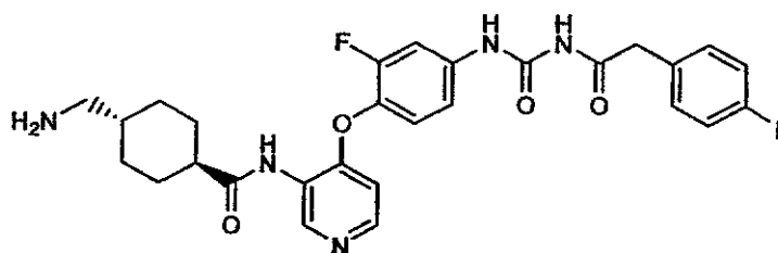
1-(4-(3-((1R,4R)-4-(Aminomethyl)cyclohexanecarboxamido)pyridin-4-yloxy)-3-fluorophenyl)-3-(2-(4-fluorophenyl)acetyl)urea
