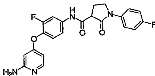
N -(4-(2-Aminopyridin-4-yloxy)-3-fluorophenyl)-1-(4-fluorophenyl)-2-oxopyrrolidine-3-carboxamide
