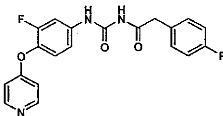
1-(3-Fluoro-4-(pyridin-4-yloxy)phenyl)-3-(2-(4-fluorophenyl)acetyl)urea
