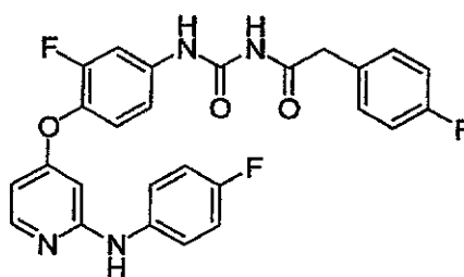
1-(3-Fluoro-4-(2-(4-fluorophenylamino)pyridin-4-yloxy)phenyl)-3-(2-(4-fluorophenyl)acetyl)urea
