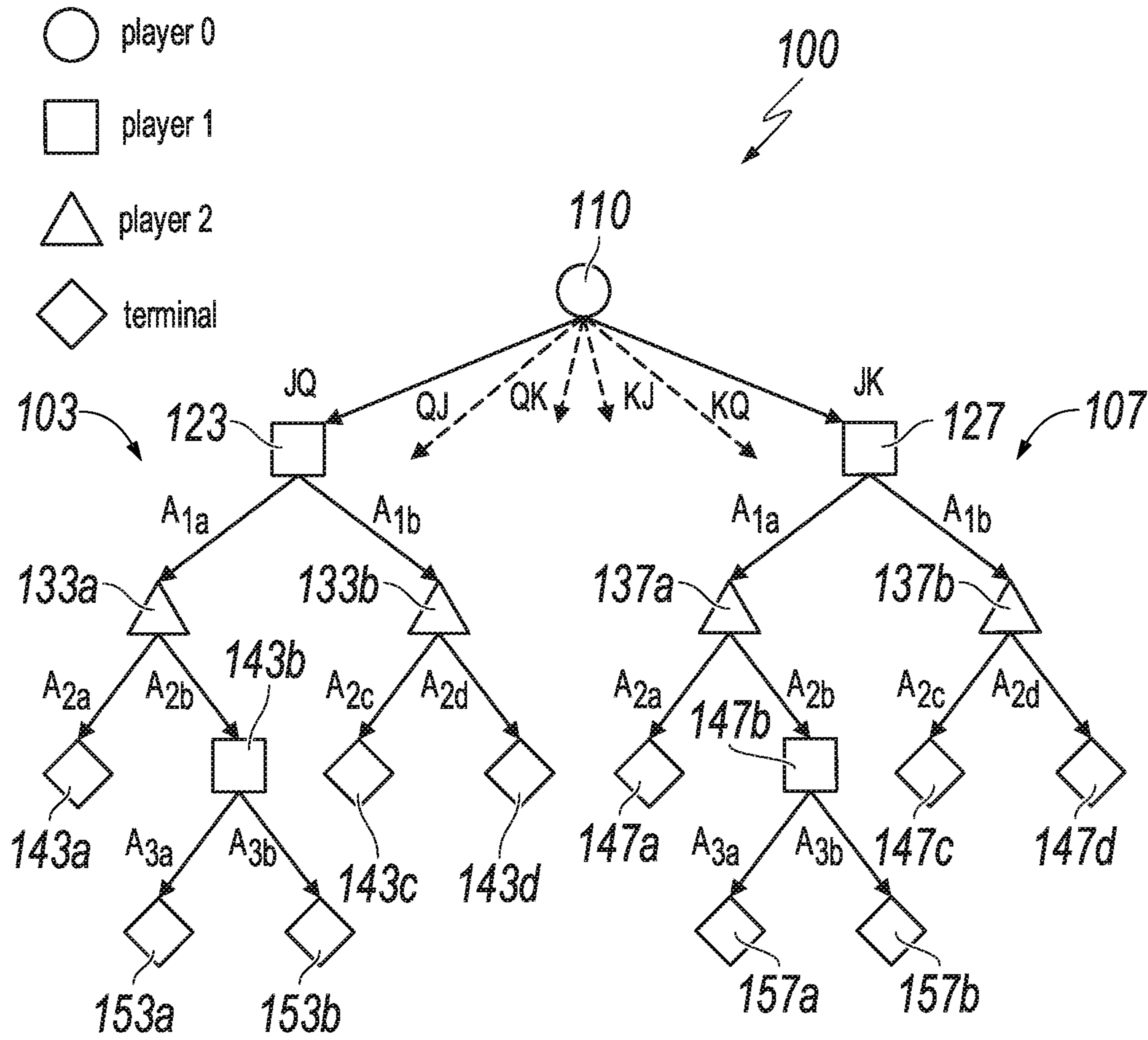
Game Tree
