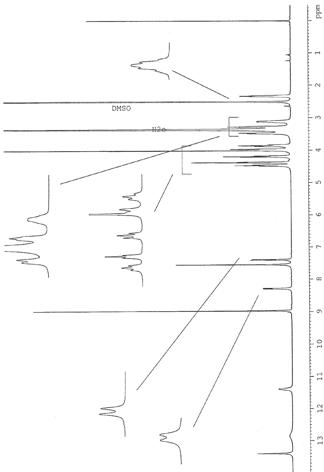
^1\text{H} -NMR Spectrum of the dihydrochloride of formula (II)
