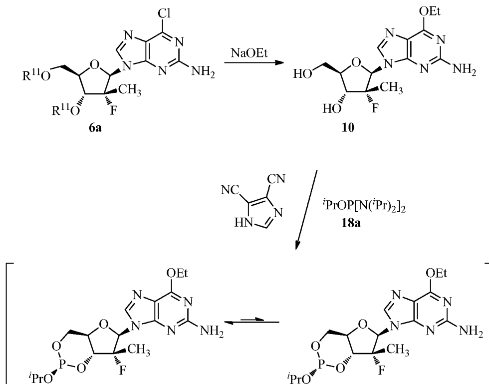
Scheme 2. Cyclic Phosphate Nucleotide By P(III)-Reagent
