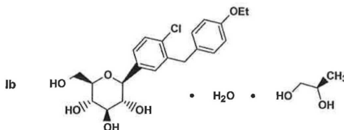
(R)-propylene glycol
