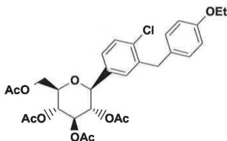
Compound A
