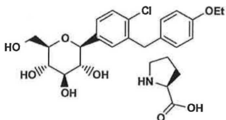
Compound Ii ;
