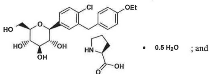
Compound Ij
