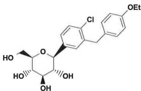
Compound I
