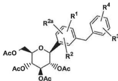
Compound C
