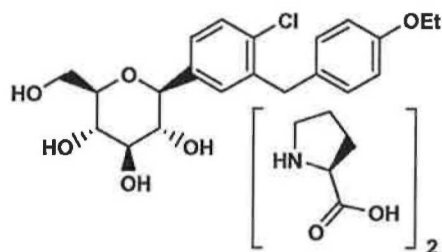
Compound Ih ;
