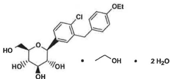
Compound Ic
