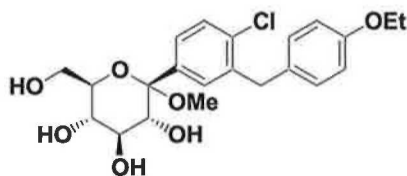
Compound B
