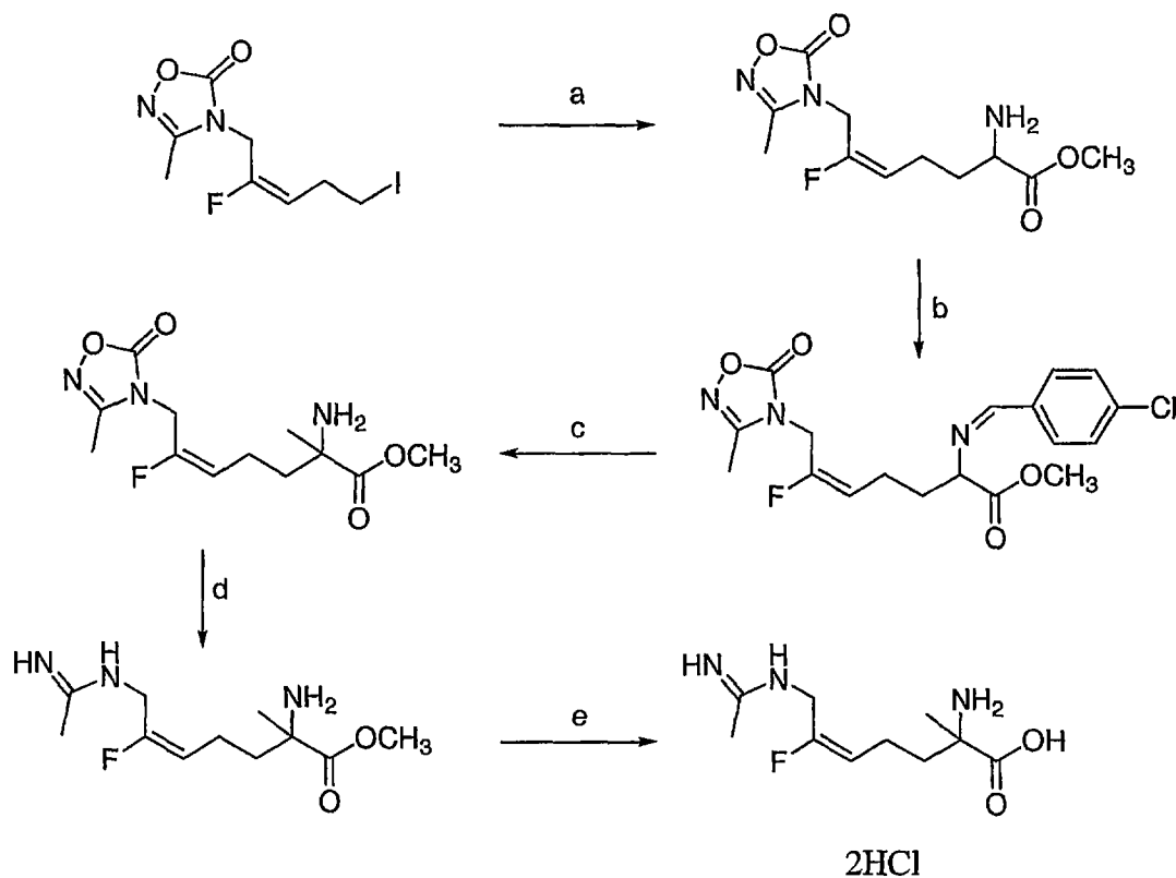
Scheme 5
