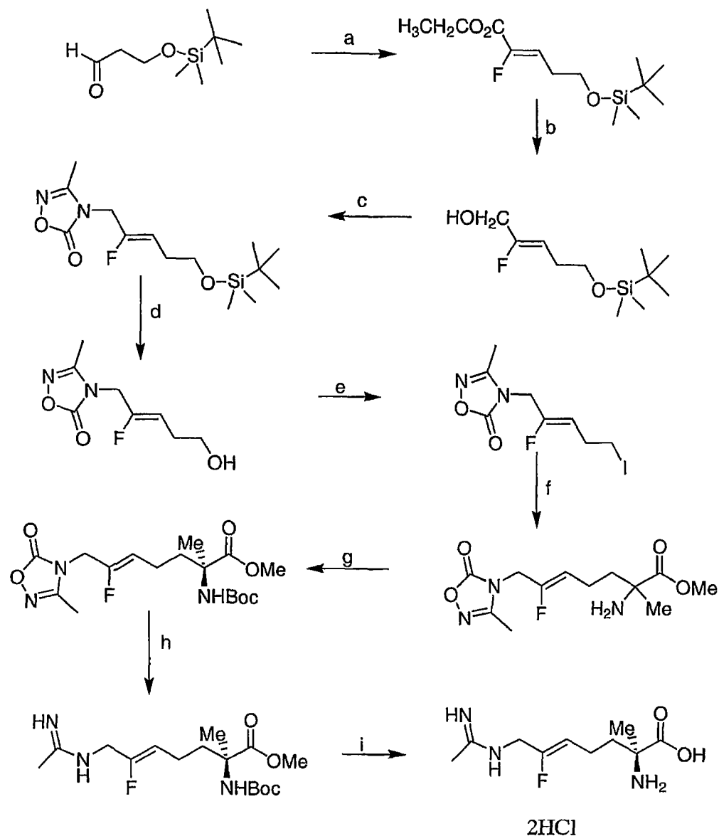
Scheme 9
