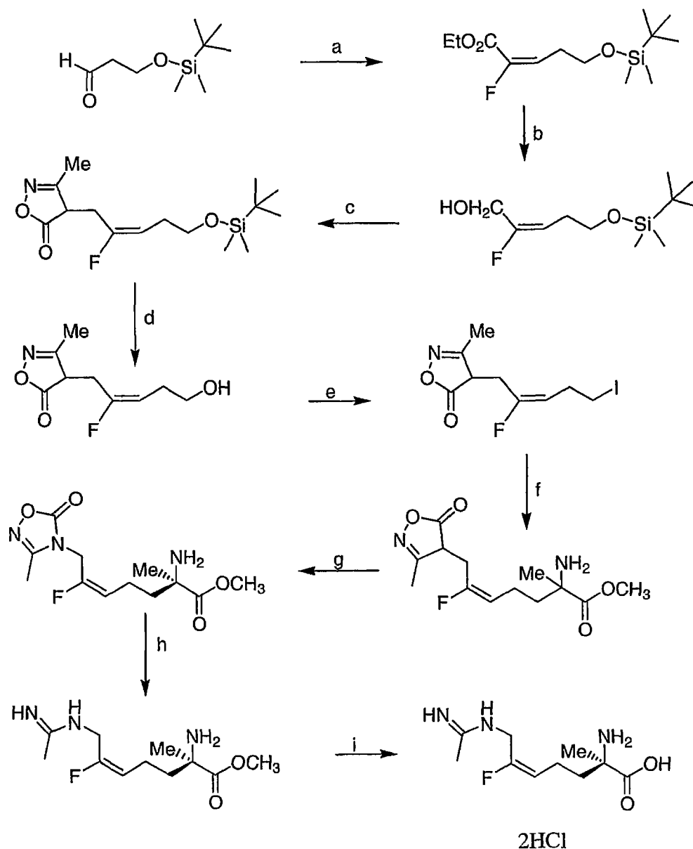
Scheme 4
