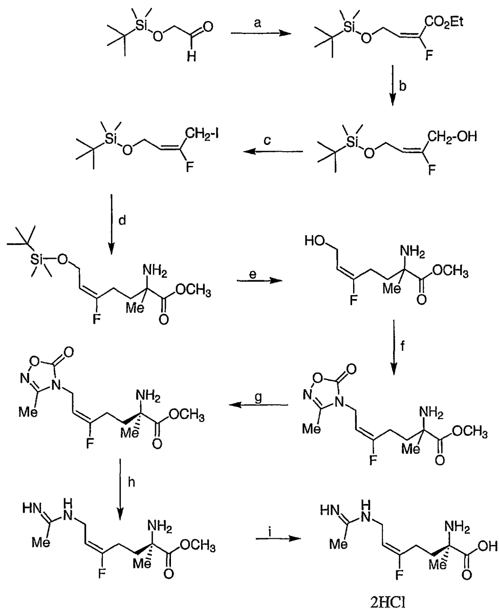
Scheme 6
