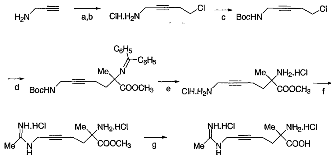
Scheme 13
