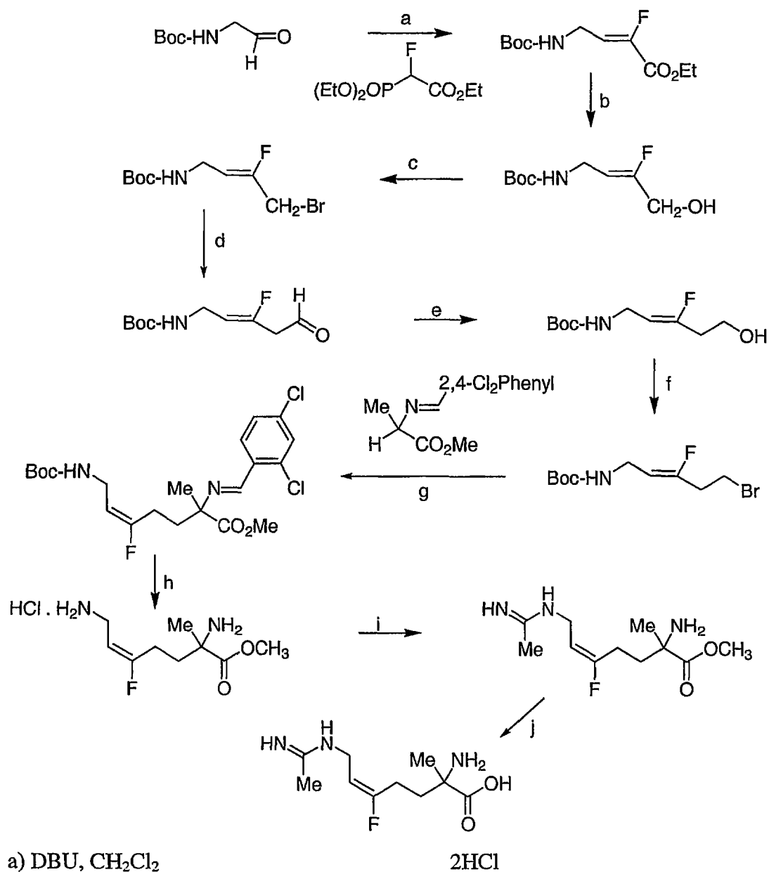
Scheme 7
