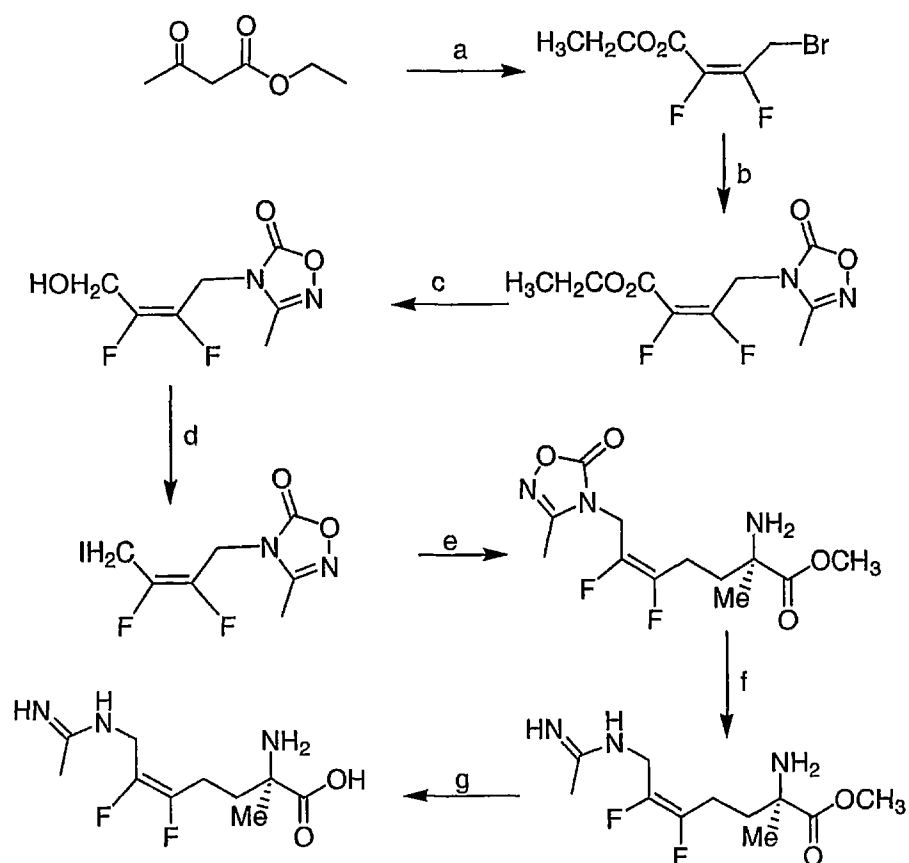
Scheme 8
