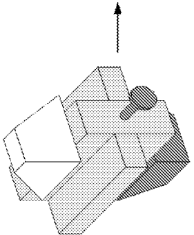
End effector in upright position ready to put twist-lock into holder
