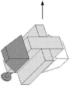
Twist-lock taken out of corner casting by end effector (turned 90 degrees)
