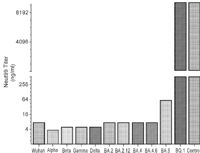
Fig. 4B SARS-CoV2 Live Virus Neutralization NVX.425.6
