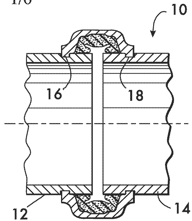
FIG. 1 PRIOR ART
