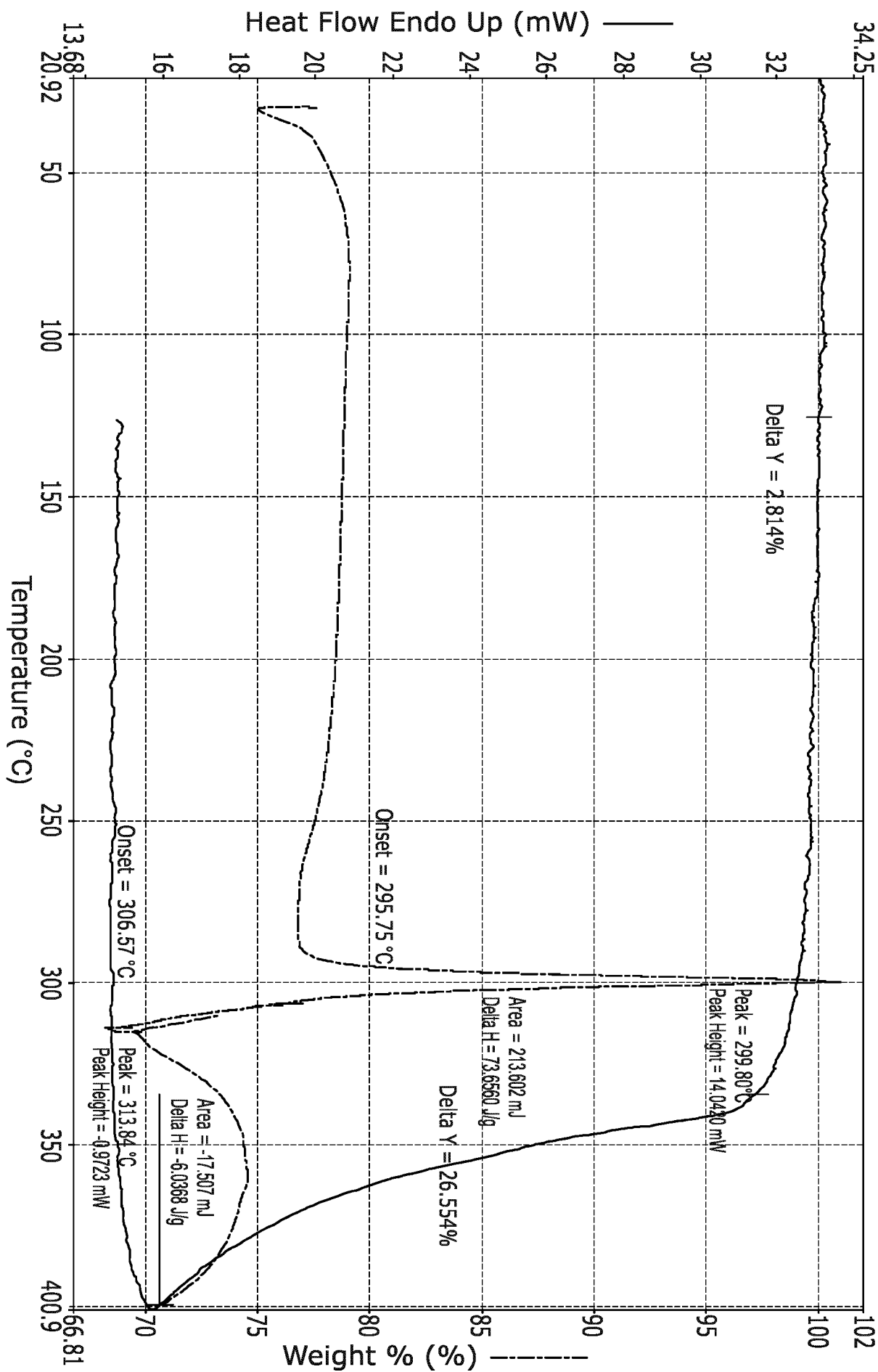
Figure 2: TGA and DSC of Form I
