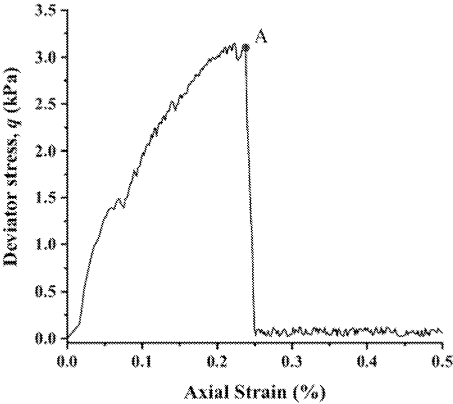
(a) Stress-strain response
