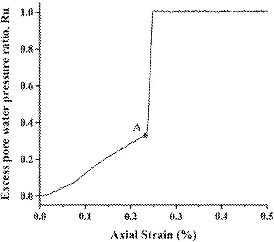
(b) Pore water pressure response
