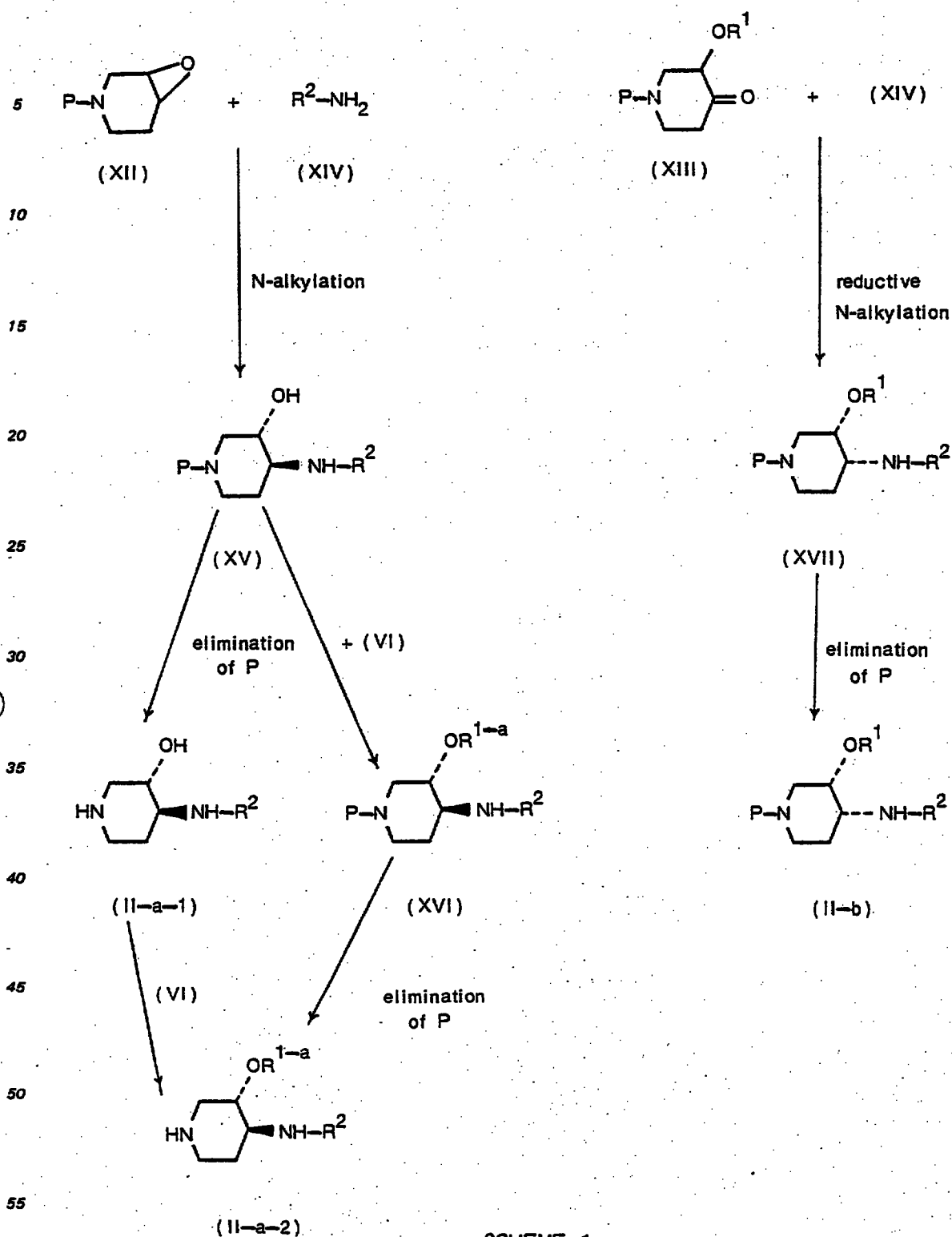
SCHEME 1
