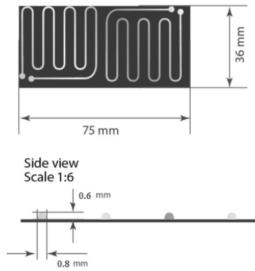
Fabric sample with design "Heating element"
