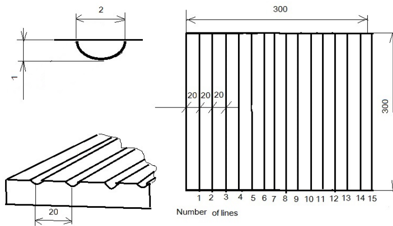
Sample with design "Lines"
