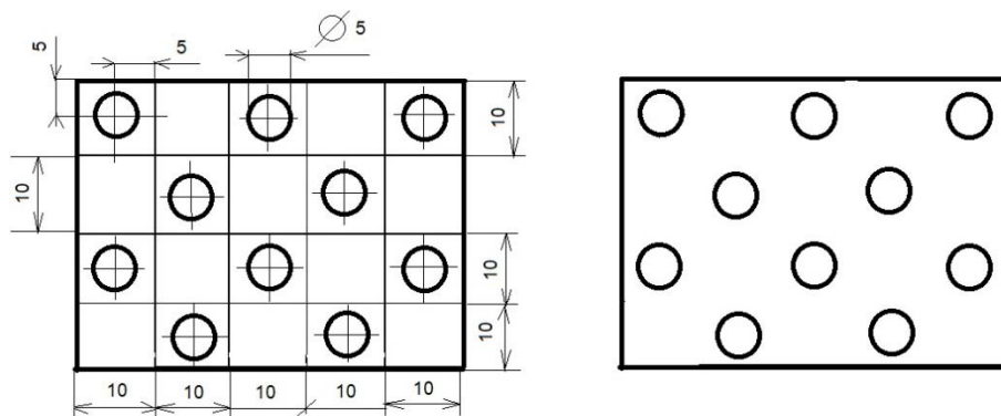
Mold for the design "Dots"
