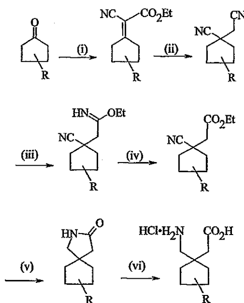
General Scheme 1
