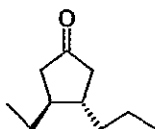
(3S,4S)-3-n-Pr-4-Et-cyclopentanone
