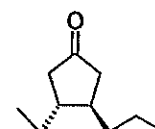
(3R,4R)-3-n-Pr-4-Et-cyclopentanone
