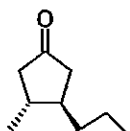
(3R,4R)-3-Methyl-4-propyl-cyclopentanone
