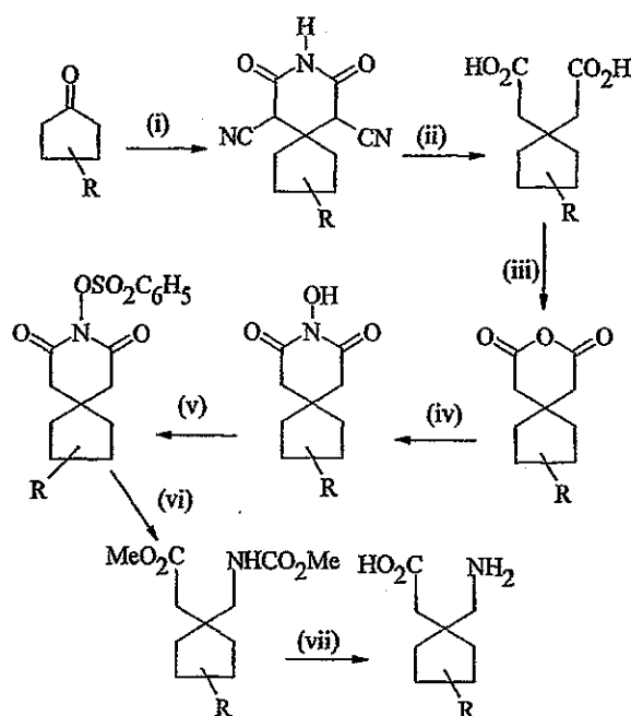
General Scheme 4
