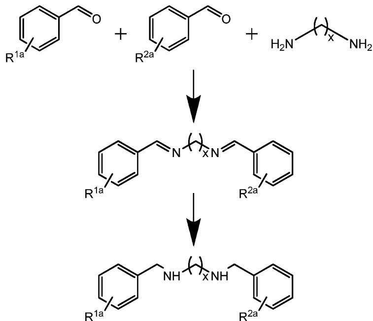
5 Scheme I
