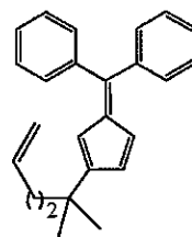
2-(1,1-dimethylpent-4-enyl)-6,6-diphenylpentafulvene
