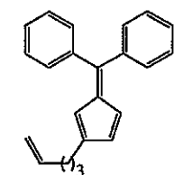
2-(pent-4-enyl)-6,6-diphenylpentafulvene
