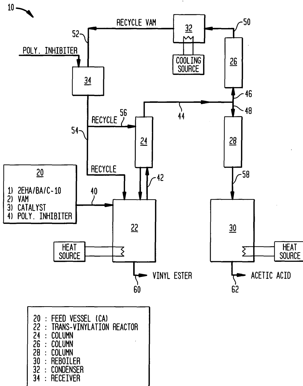
FIG. 1 SEMI CONTINUOUS TRANS-VINYLATION PROCESS
