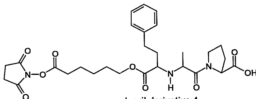
eanalapril derivative 4
