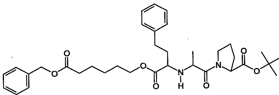
eanalapril derivative 1
