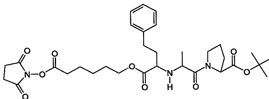
eanalapril derivative 3
