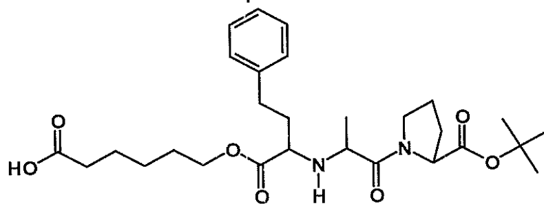
eanalapril derivative 2
