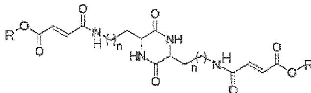
Formula I
