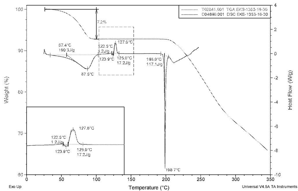
Figure 2. TGA and DSC of Form D
