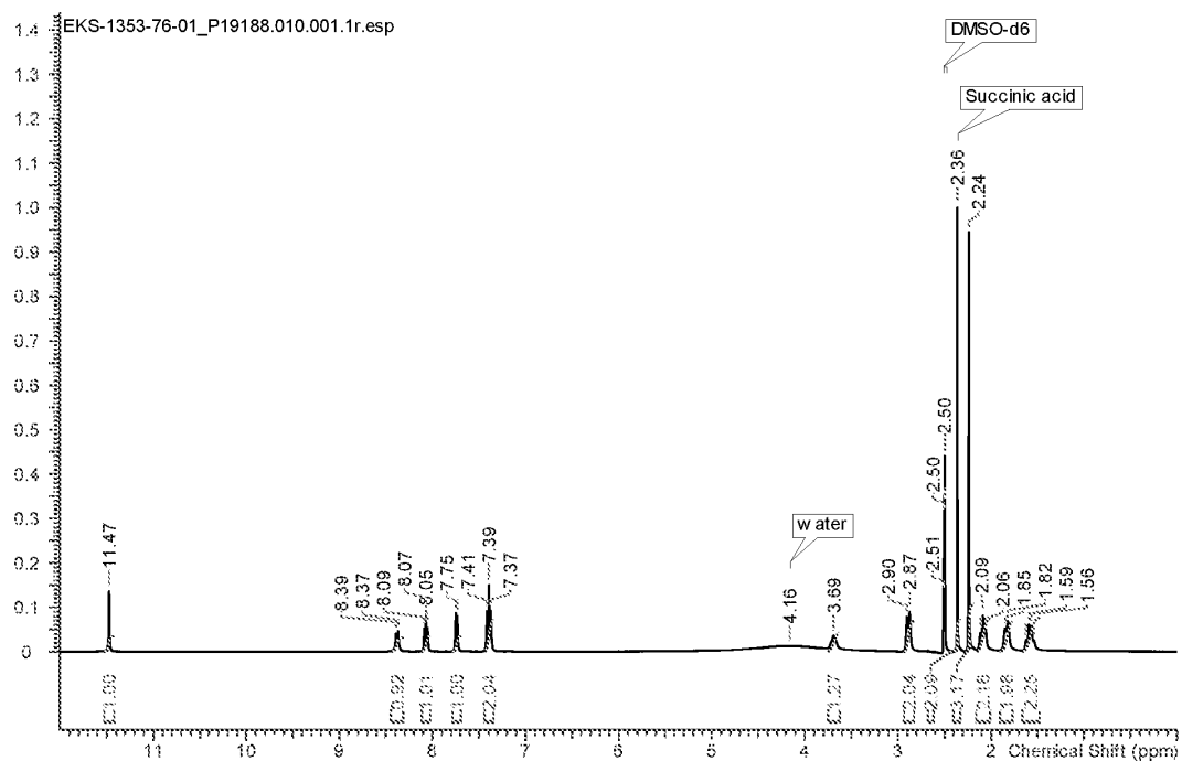
Figure 5. The solution state 1 H-NMR spectrum of dissolved Form D or F of Compound I.
