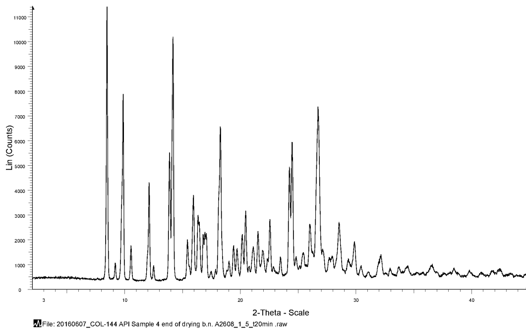
Figure 1C. XRPD of Form E of Compound I
