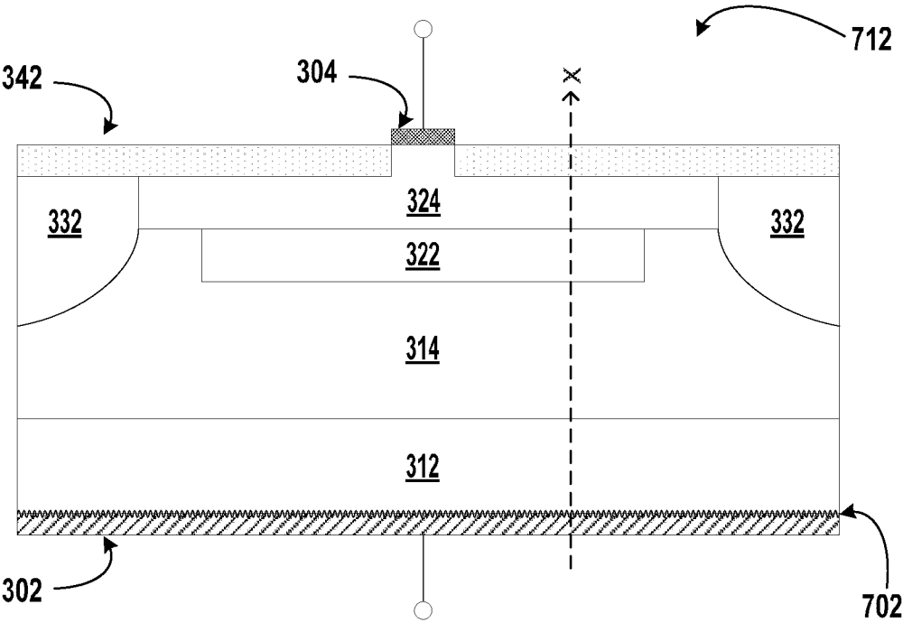
Side View
