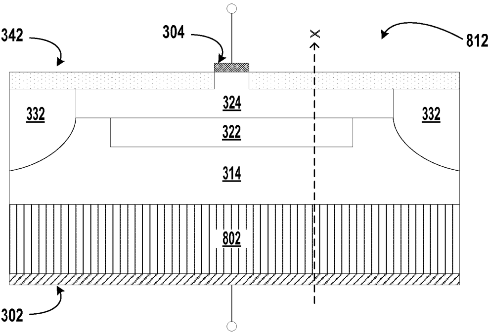
Side View
