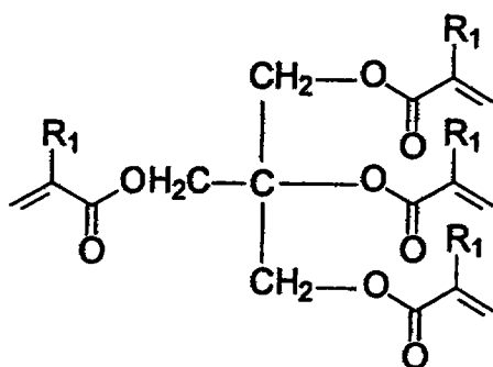
pentaerythritol tetraacylate and tetramethacrylate
