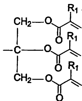
glyceryl triacrylates and trimethacrylates
