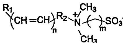
polyunsaturated sulfo-betaines
