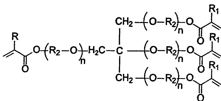
alkoxylated pentaerythritol tetraacylate and tetramethacrylate
