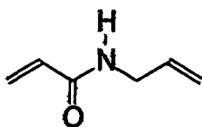
allyl acrylamide
