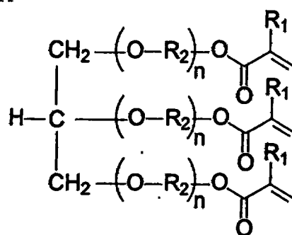
alkoxylated glyceryl triacylate and trimethacrylate
