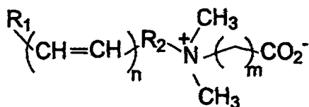
polyunsaturated betaines
