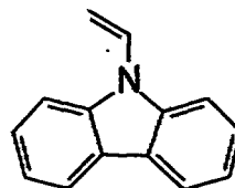
N-vinylcarbazole
