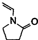
N-vinyl pyrrolidone
