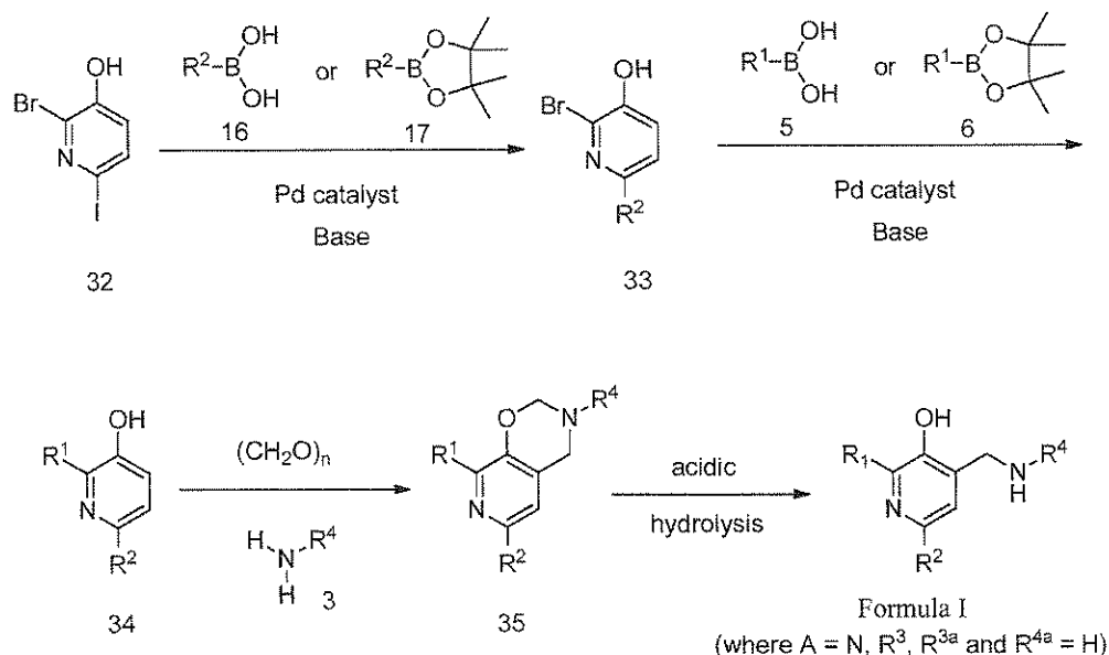
Scheme 12
