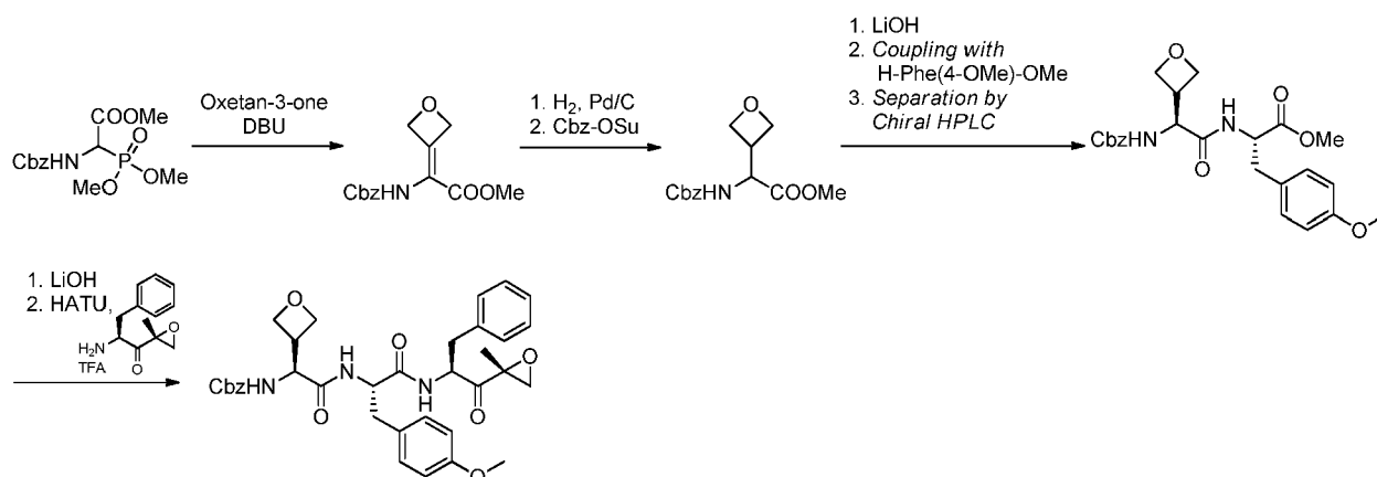
Methyl 2-(benzyloxycarbonylamino)-2-(oxetan-3-ylidene)acetate
