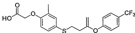
Compound 20
