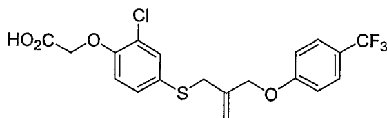
Compound 11
