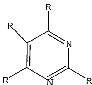
Pyrimidine
