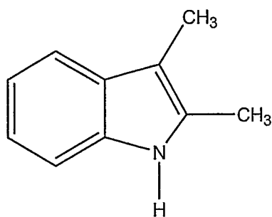
2,3-dimethyl indole
