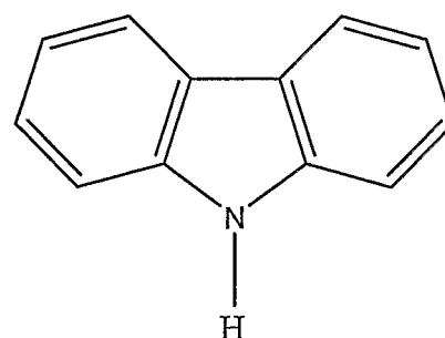
Carbazole
