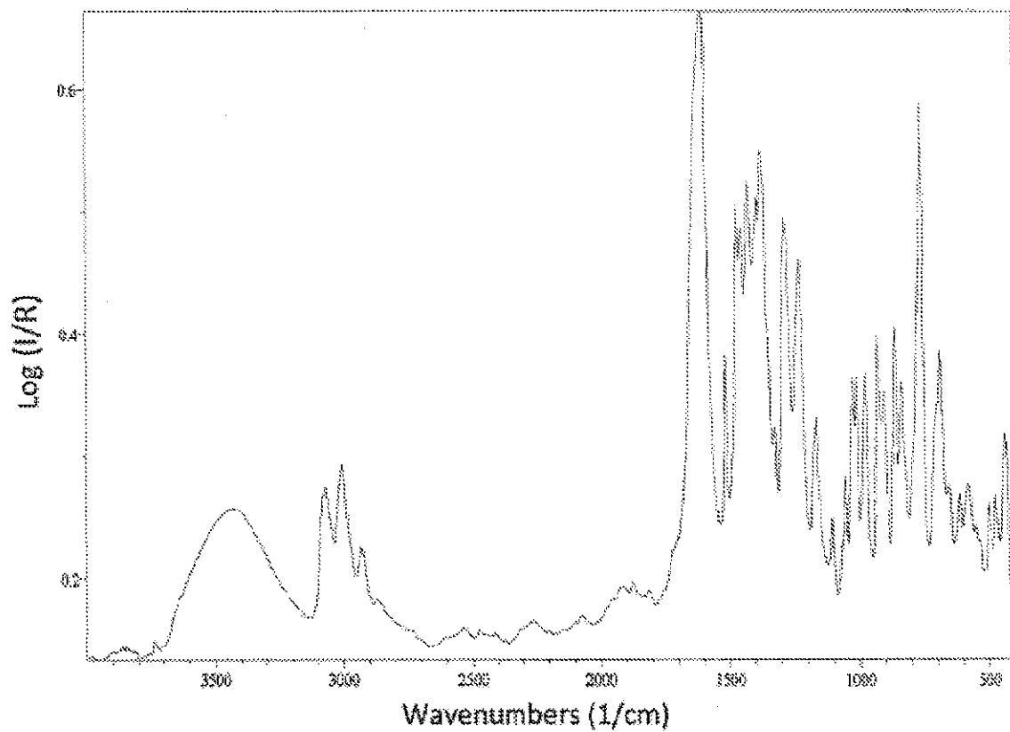
FIGURE 3 Sodium 2-(5-bromo-4-(4-cyclopropynaphthalen-1-yl)-4H-1,2,4-triazol-3-ylthio)acetate, Polymorph Form A: IR spectrum
