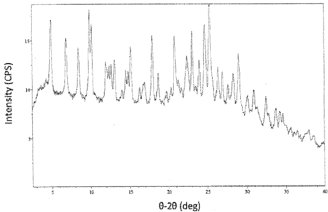
FIGURE 1 Sodium 2-(5-bromo-4-(4-cyclopropylnaphthalen-1-yl)-4H-1,2,4-triazol-3-ylthio)acetate, Polymorph Form A: X-ray Powder Diffraction Pattern
