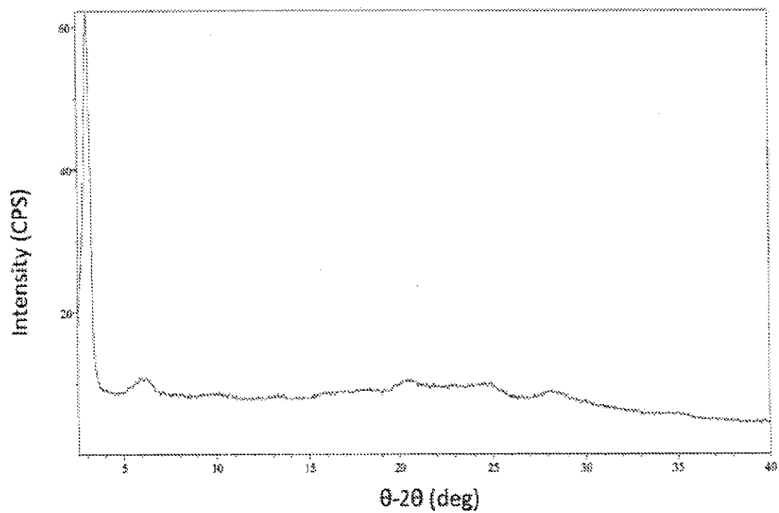
FIGURE 14 Sodium 2-(5-bromo-4-(4-cyclopropylnaphthalen-1-yl)-4H-1,2,4-triazol-3-ylthio)acetate, X-ray Powder Diffraction Mesophase Pattern 2
