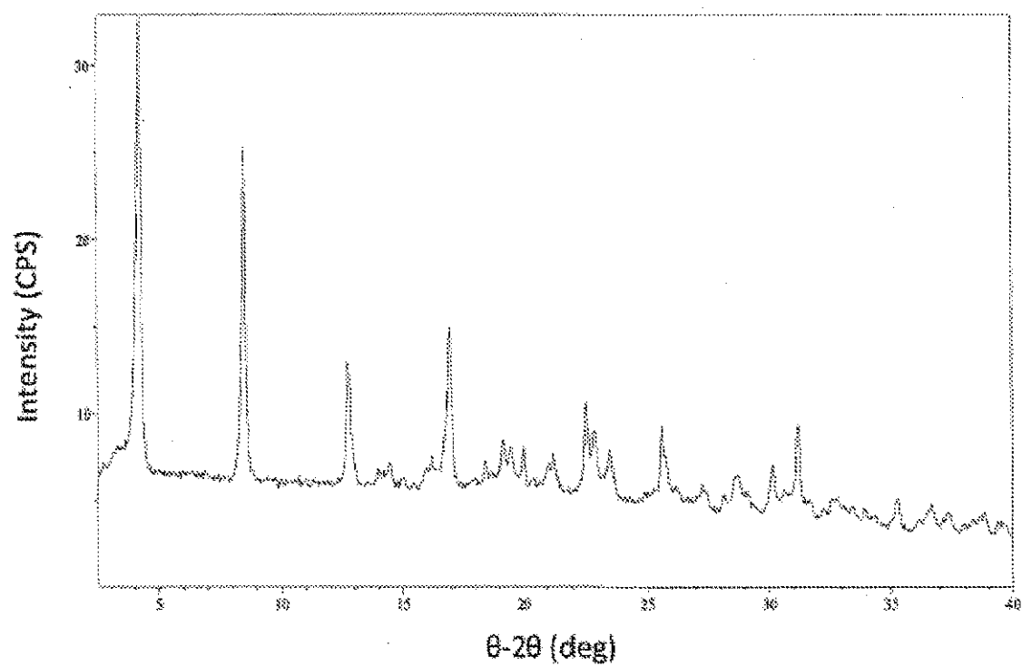
FIGURE 5 Sodium 2-(5-bromo-4-(4-cyclopropyl)naphthalen-1-yl)-4H-1,2,4-triazol-3-ylthio)acetate, Polymorph Form B: X-ray Powder Diffraction Pattern
