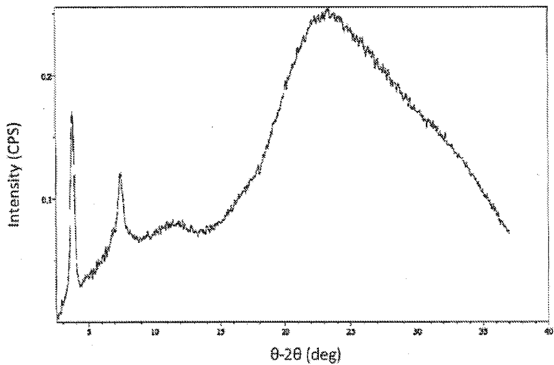
FIGURE 15 Sodium 2-(5-bromo-4-(4-cyclopropylnaphthalen-1-yl)-4H-1,2,4-triazol-3-ylthio)acetate, X-ray Powder Diffraction Mesophase Pattern 3
