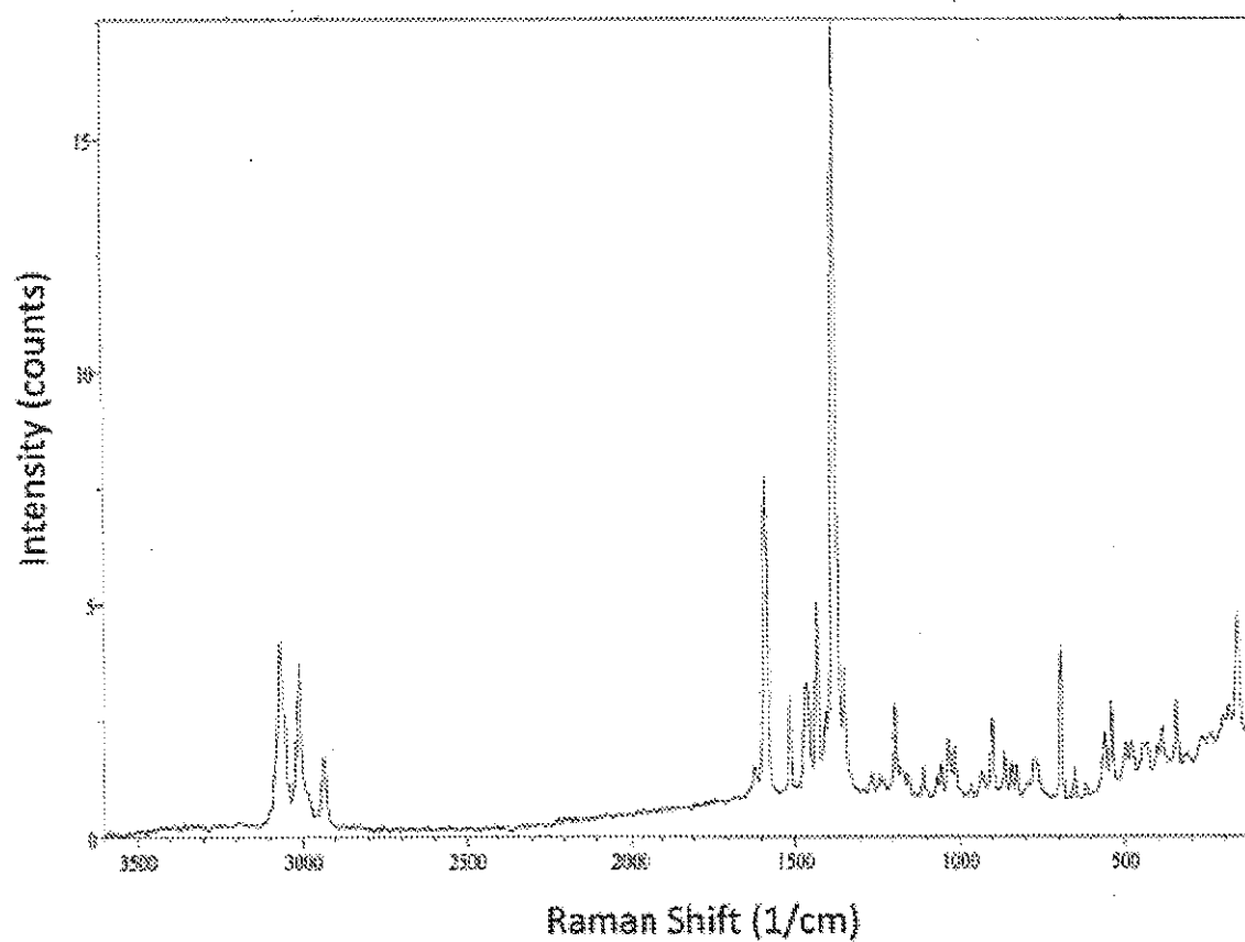
FIGURE 4 Sodium 2-(5-bromo-4-(4-cyclopropyl-naphthalen-1-yl)-4H-1,2,4-triazol-3-ylthio)acetate, Polymorph Form A: Raman spectrum
