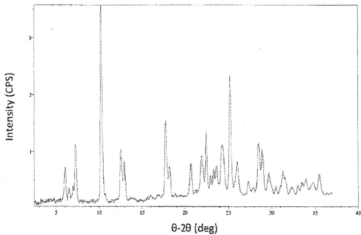
FIGURE 10 Sodium 2-(5-bromo-4-(4-cyclopropyl-naphthalen-1-yl)-4H-1,2,4-triazol-3-ylthio)acetate, X-ray Powder Diffraction Pattern D
