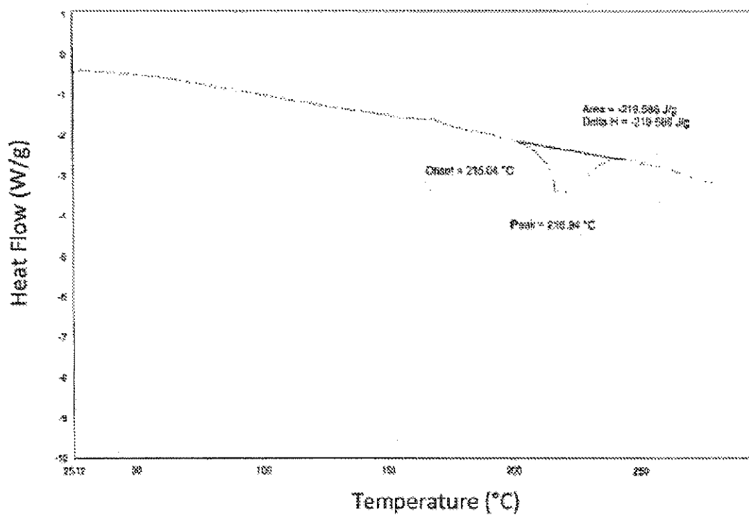
FIGURE 8 Sodium 2-(5-bromo-4-(4-cyclopropynaphthalen-1-yl)-4H-1,2,4-triazol-3-ylthio)acetate, Polymorph Form B': Differential Scanning Calorimetry
