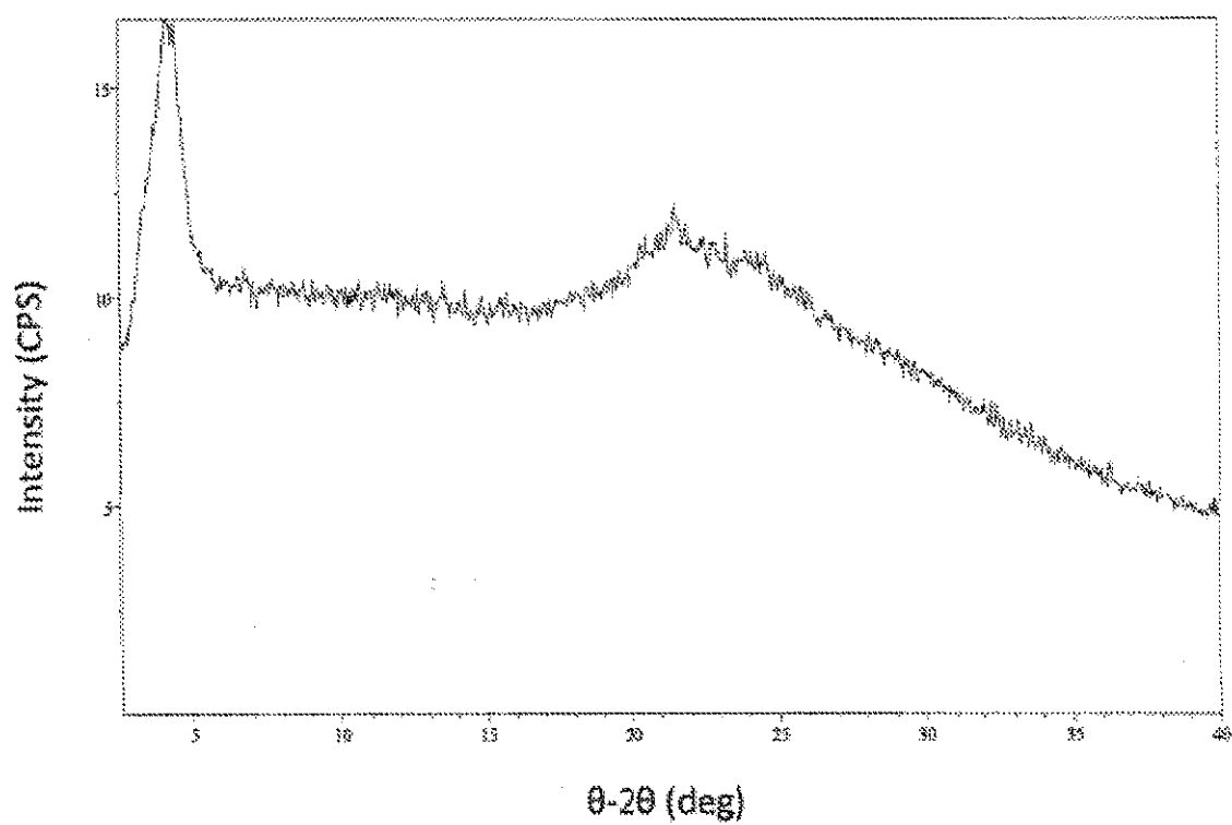
FIGURE 12 Sodium 2-(5-bromo-4-(4-cyclopropylnaphthalen-1-yl)-4H-1,2,4-triazol-3-ylthio)acetate, X-ray Powder Diffraction Mesophase Pattern 1
