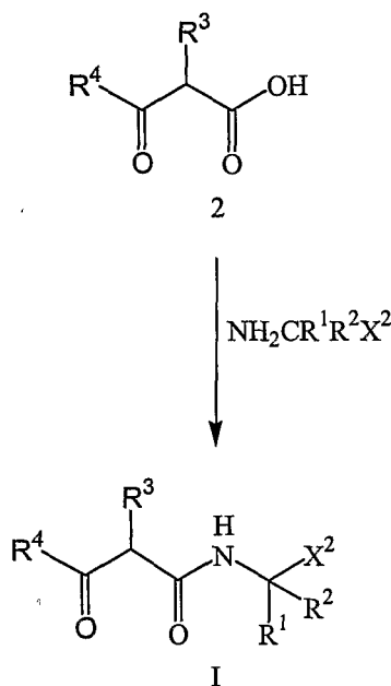
Reaction Scheme 1
