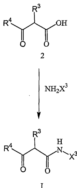
Reaction Scheme 2
