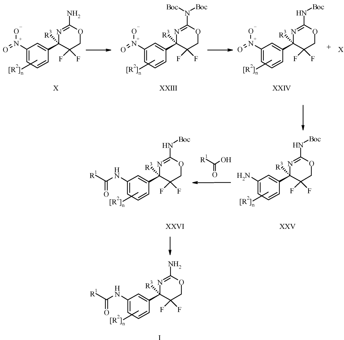
Scheme 4: Synthesis of compounds of formula I with R^4, R^5 = H
