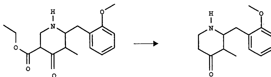
Piperidone-Ester
