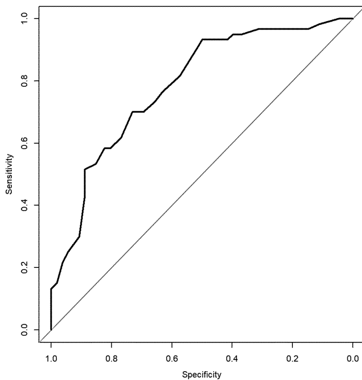
Fig. 3C. NIHSS+ N20=0.784
