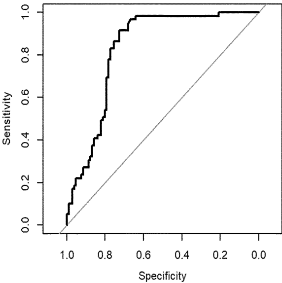
Fig. 5C. TICI+N20(log-transformed).AUC=0.829
