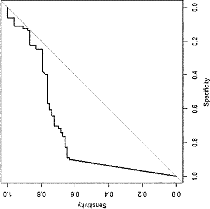
Fig. 4B. NIHSS+ASPECTS.AUC=0.697
