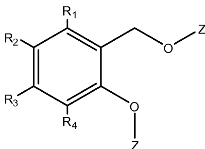
Formula Ia
