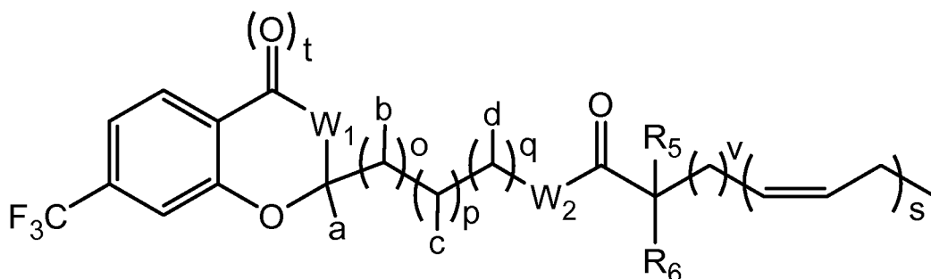
Formula VIe'
