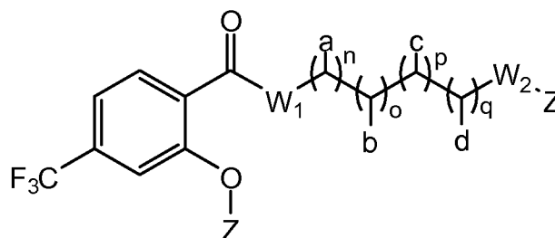
Formula VIc
