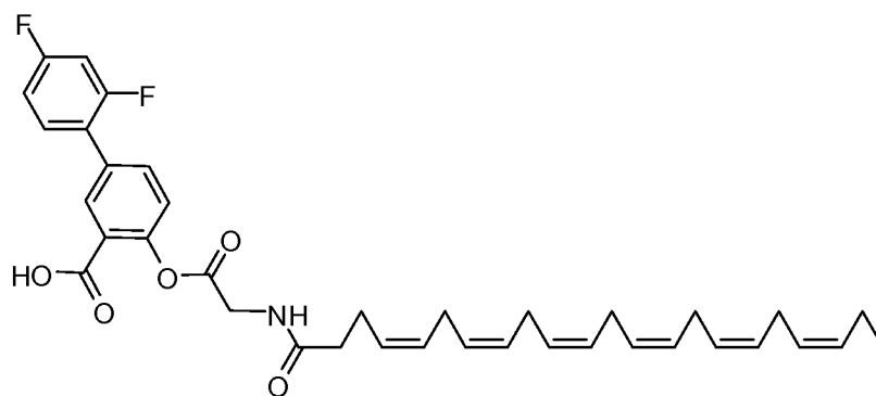
IVg-1
