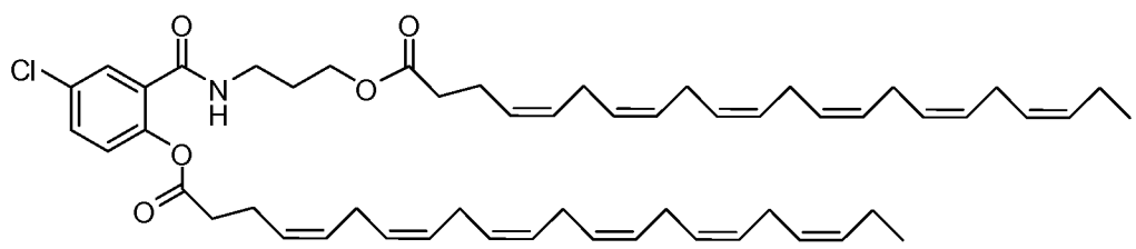
Id-2
