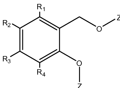
Formula Ie
