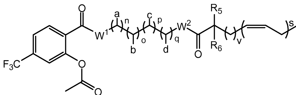
Formula VIb'
