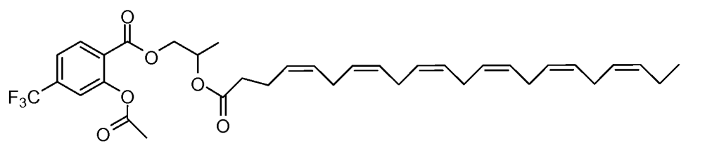
VIb-6
