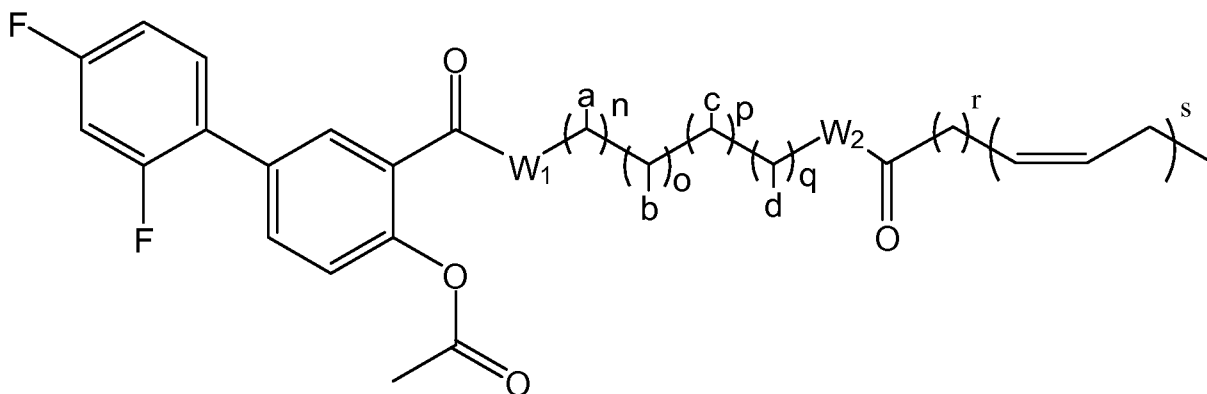
Formula IVb
