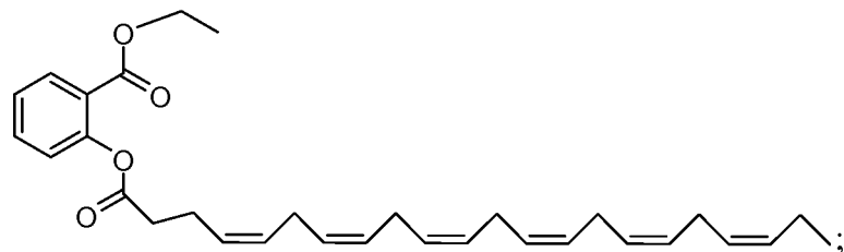
Id-4
