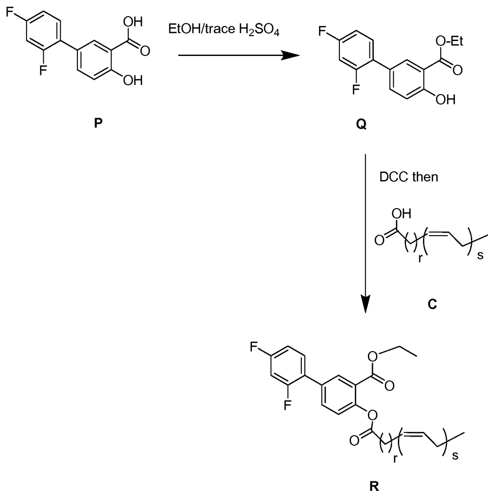
Scheme 5
