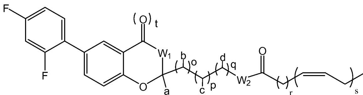
Formula IVe
