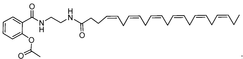
Ic-10
