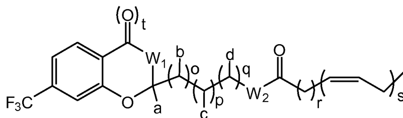
Formula VIe
