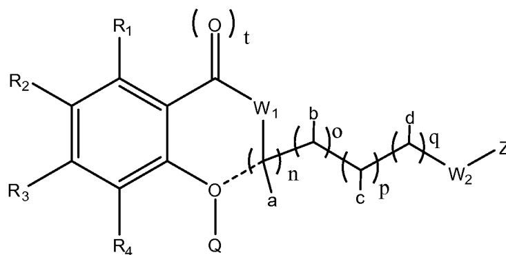
Formula II
