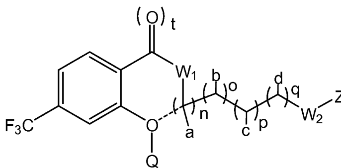
Formula VII'
