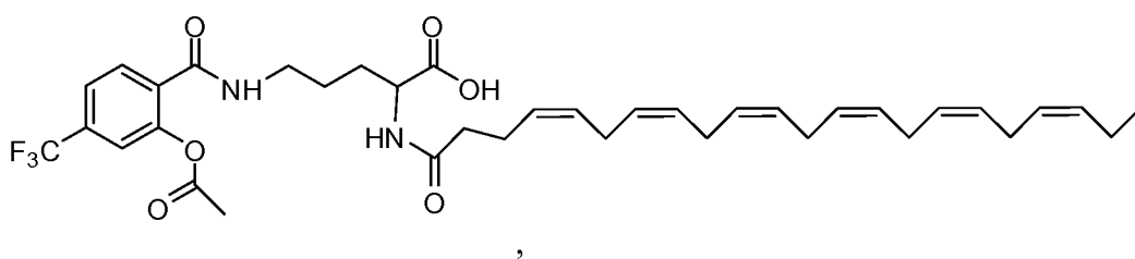
VIb-8
