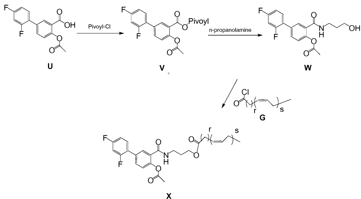
Scheme 7
