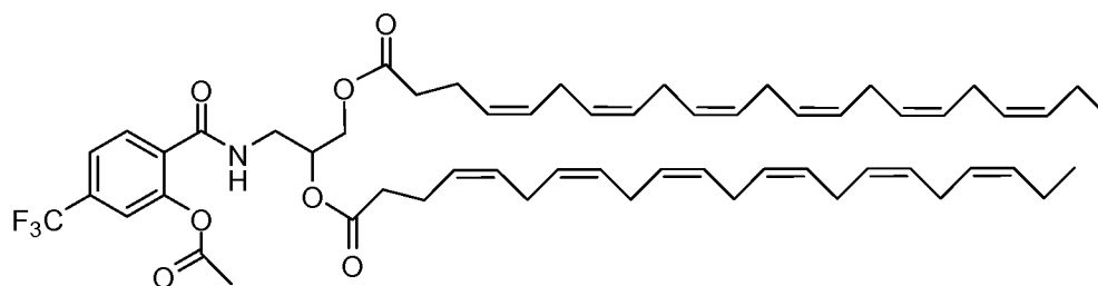
VIb-4
