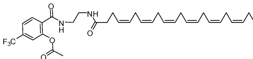
VIb-12
