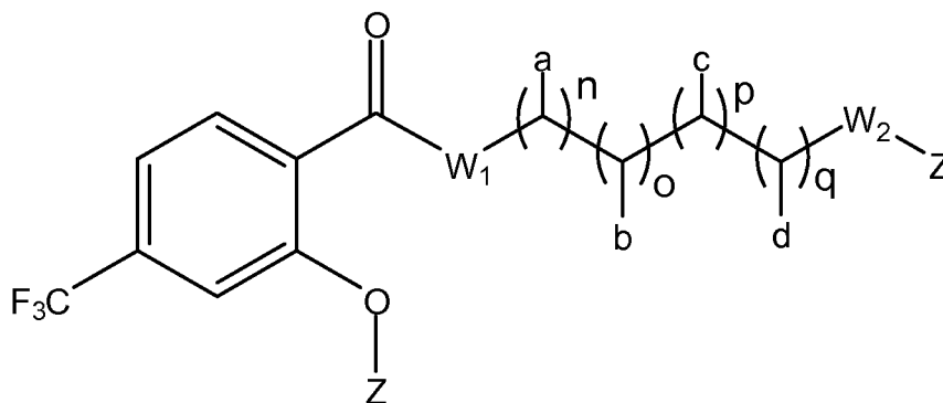
Formula VIc'
