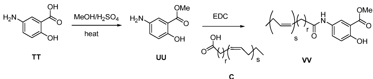
Scheme 15
