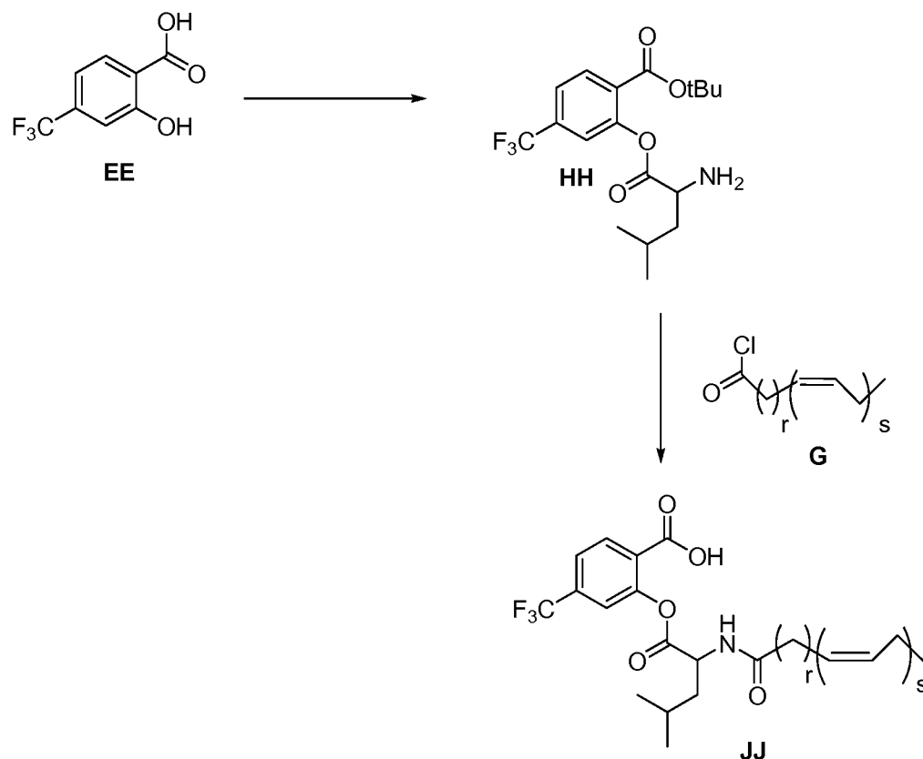
Scheme 11
