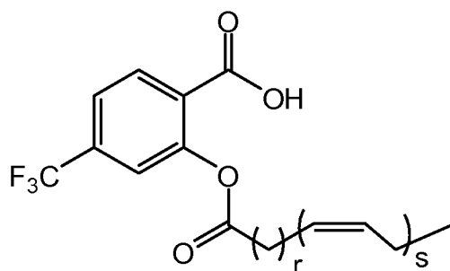
Formula VIa
