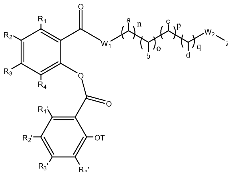
Formula Ib
