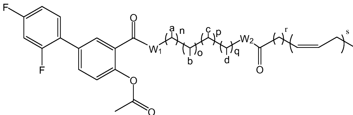
Formula IVb
