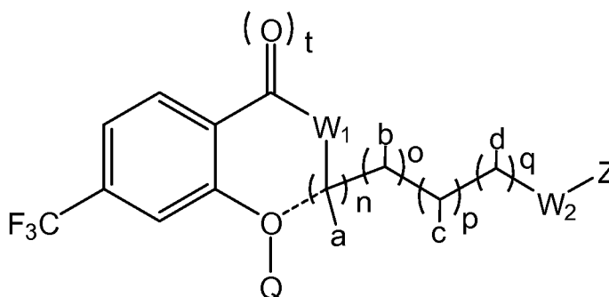
Formula VII
