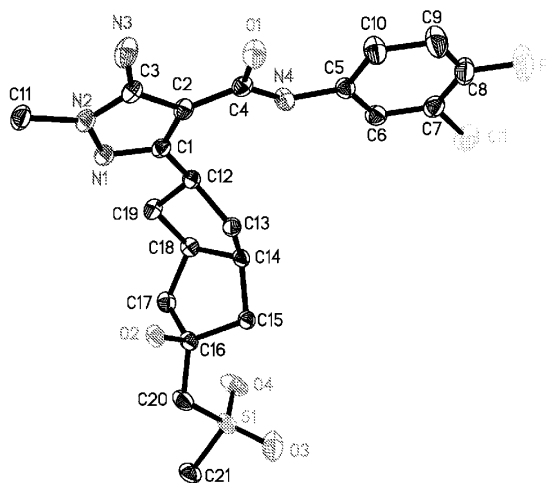
Fig. 1 The ORTEP plot for compound AIA-227-2
