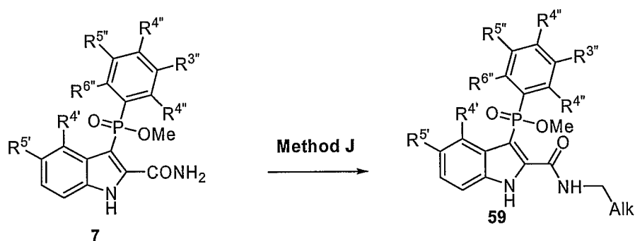
Scheme 16: Phosphinic Acids
