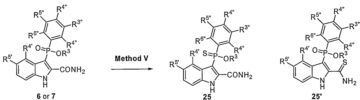
Scheme 5:
