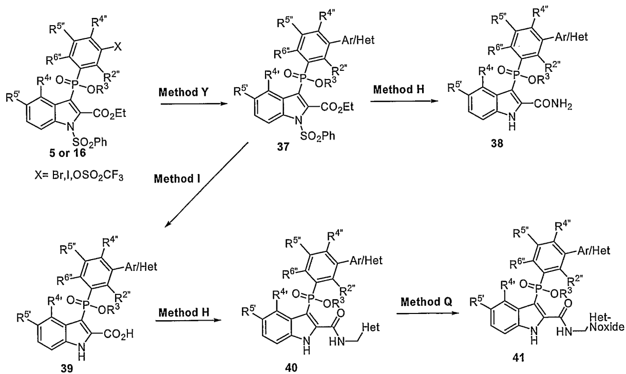
Scheme 10:
