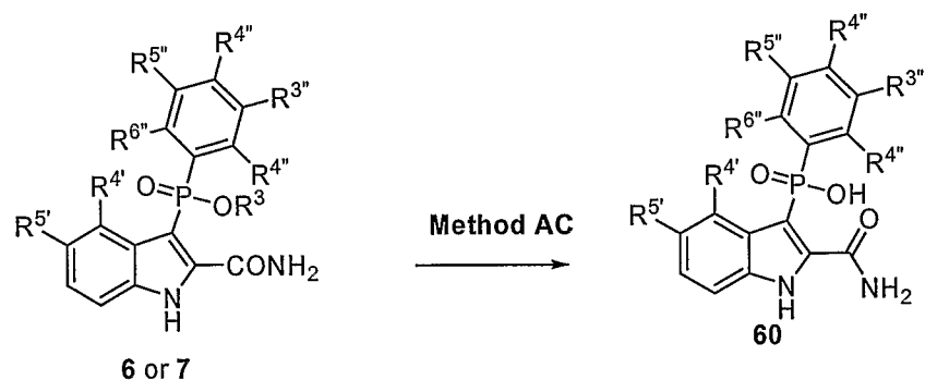
Scheme 16: Phosphinic Acids
