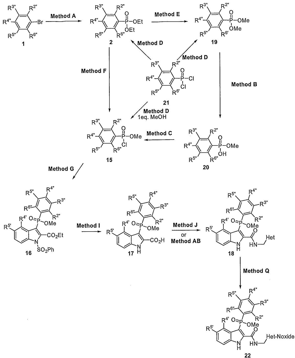
Scheme 2:
