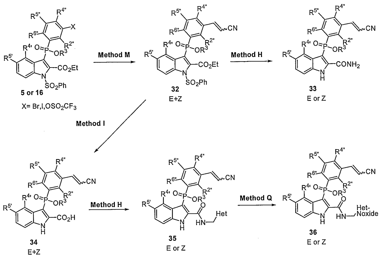
Scheme 10:
