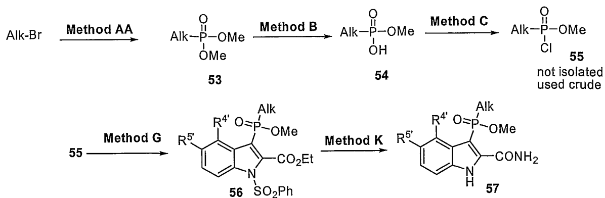
Scheme 14: Alkyl Phosphinates
