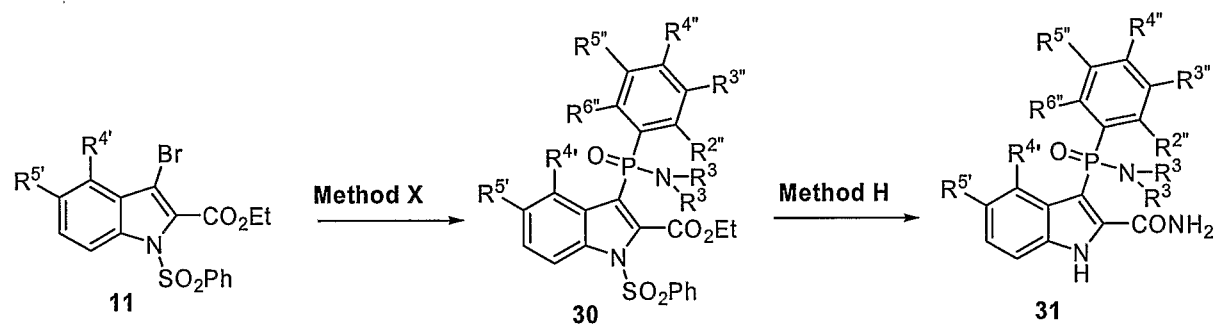
Scheme 8:
