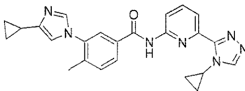
Compound B.
