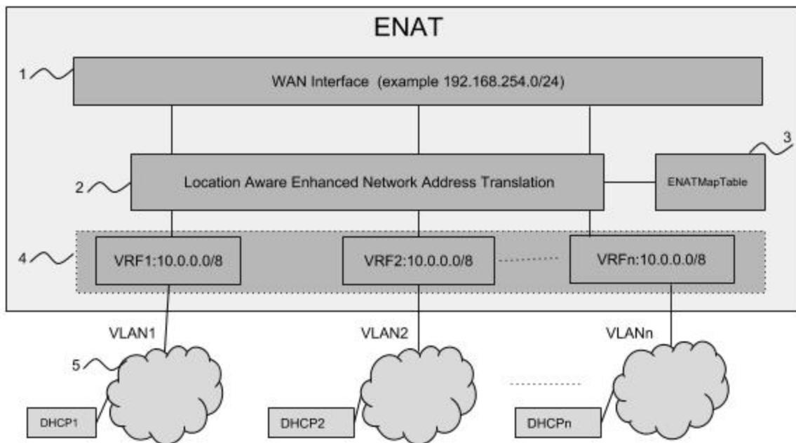
Fig 1 ENAT Architecture
