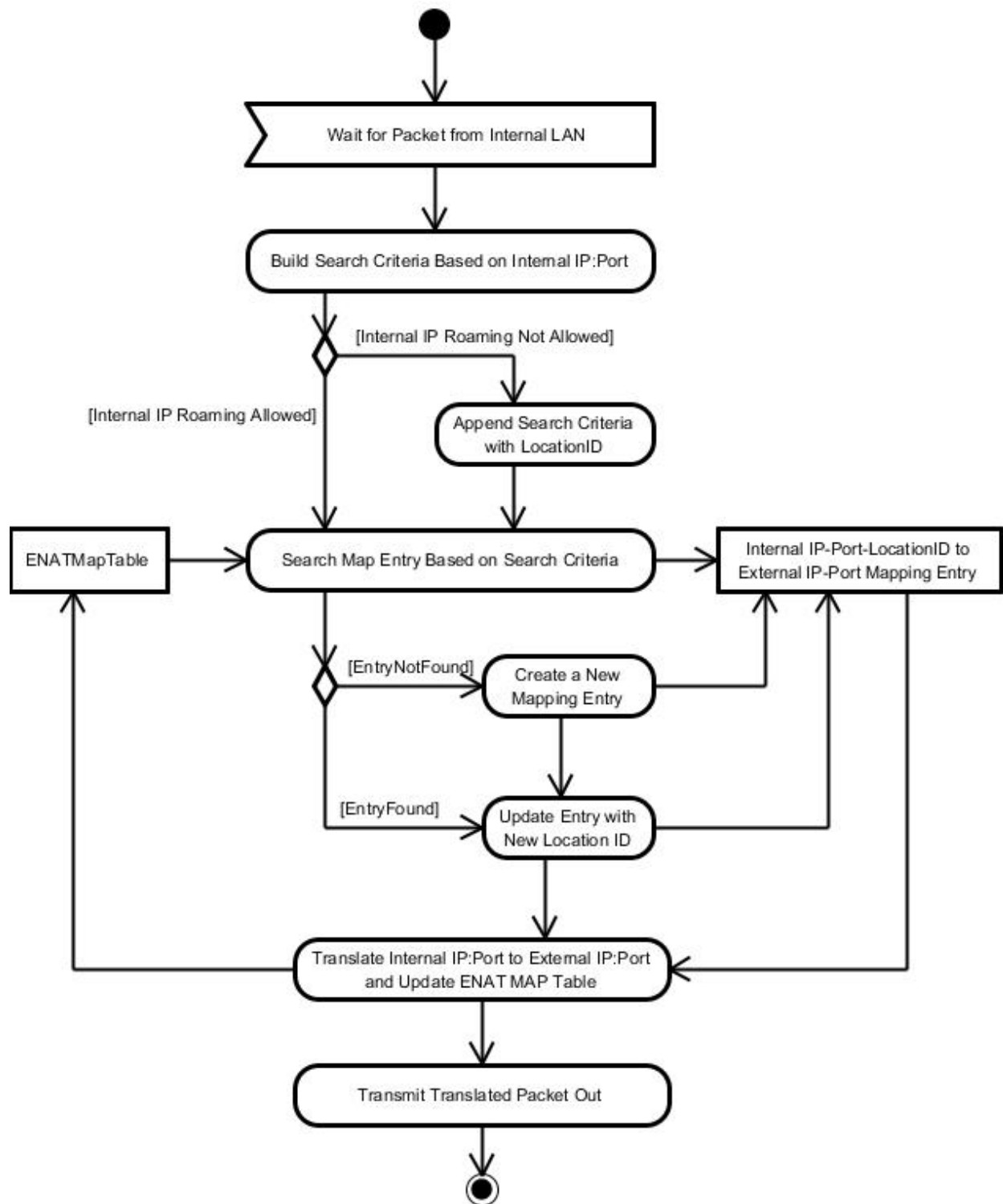
Fig 3 Ingress to LAN Packet Processing Flow
