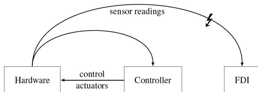
Figure 5.3: Diagram of the connection of the FDI to the test structure
