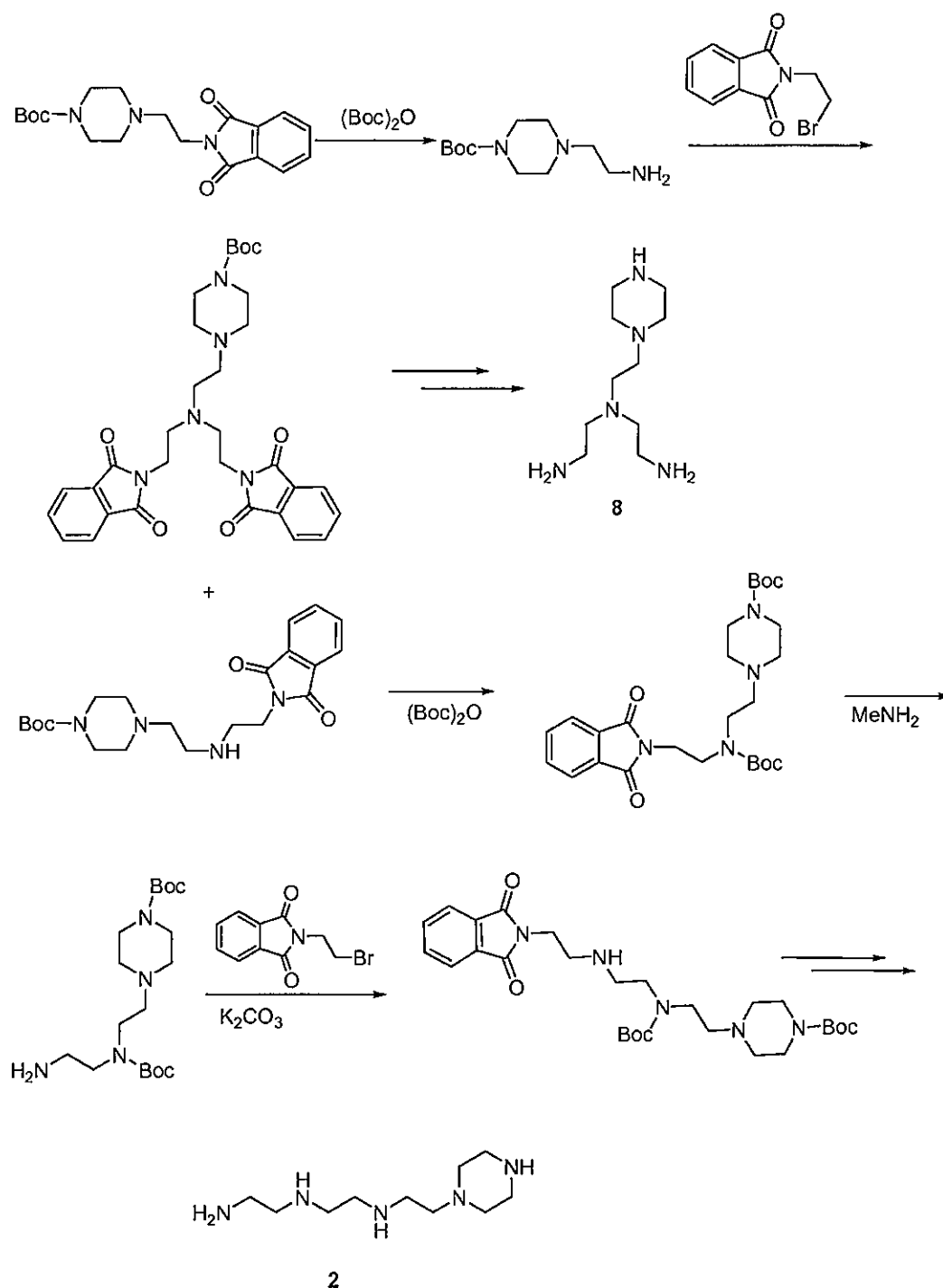
Scheme 2
