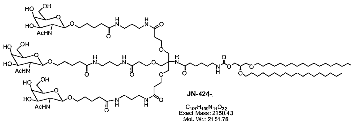
Formula 2
