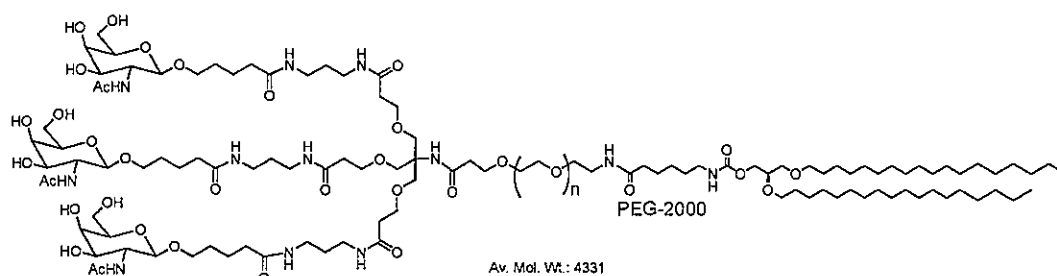
Formula 3
