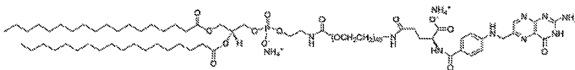
Formula 4
