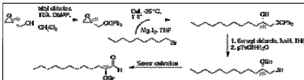
Scheme 10
