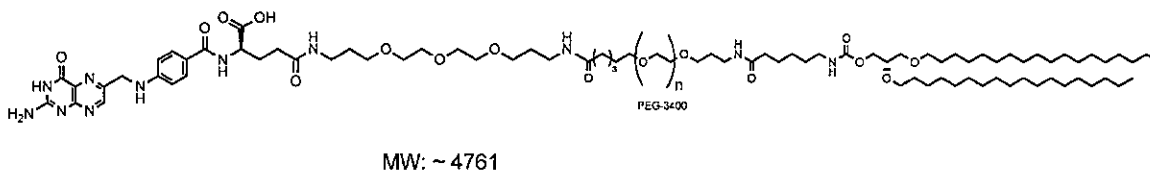
Formula 7.
