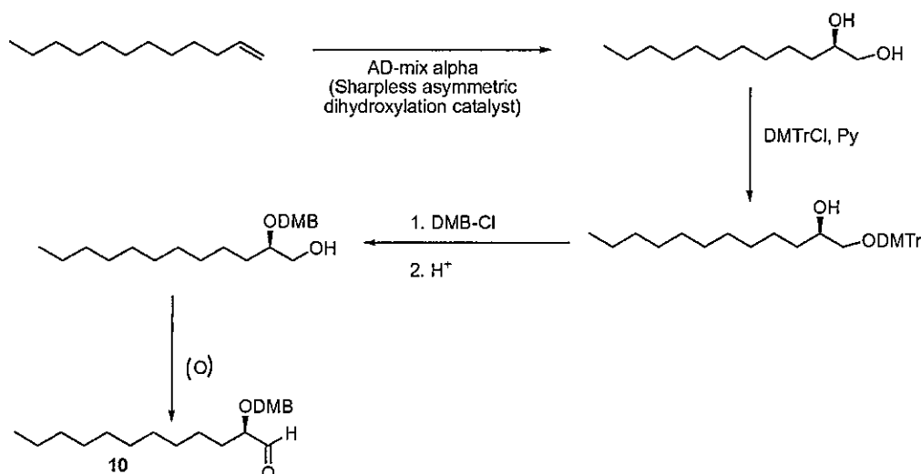
Scheme 9
