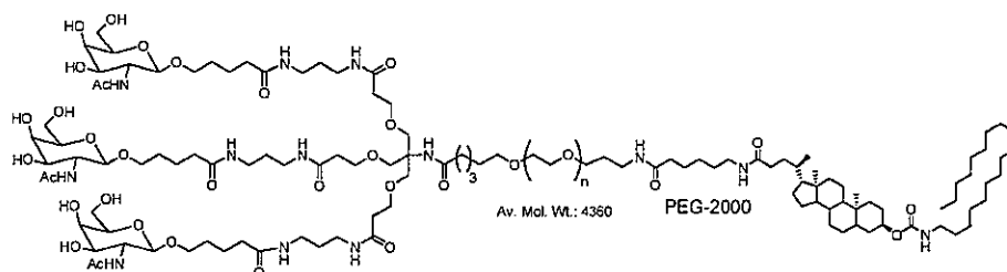
Formula 4
