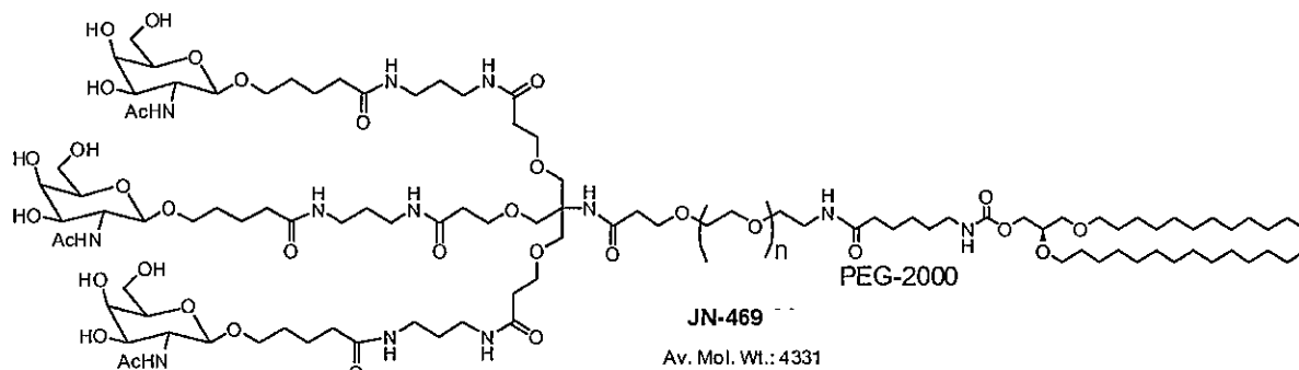
Formula 3
