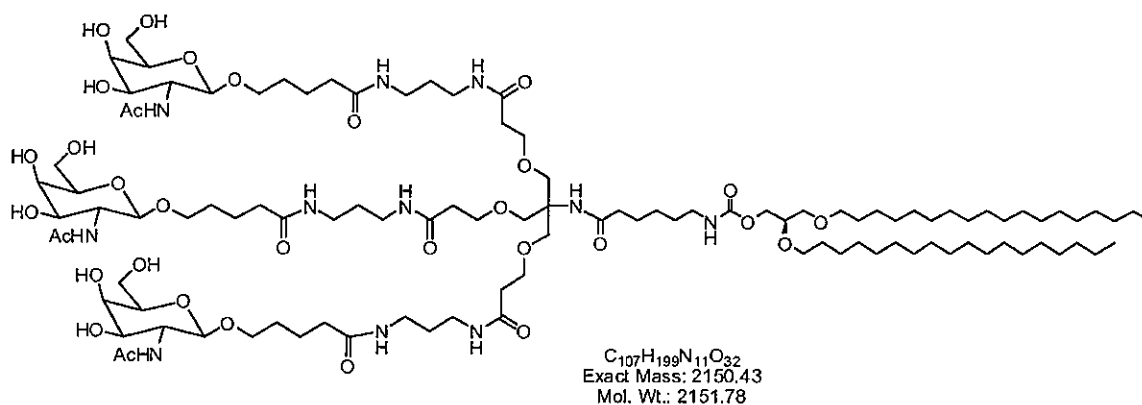
Formula 2
