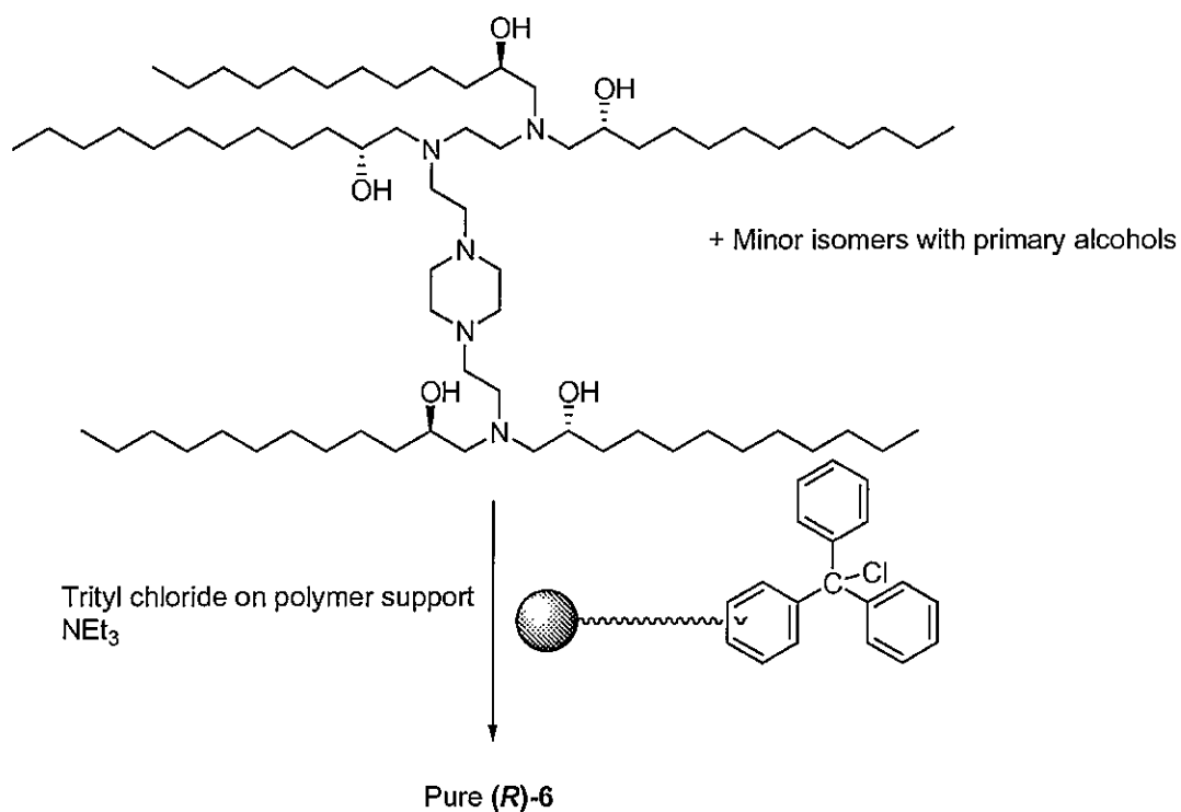
Scheme 8
