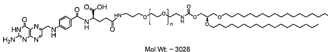
Formula 6
