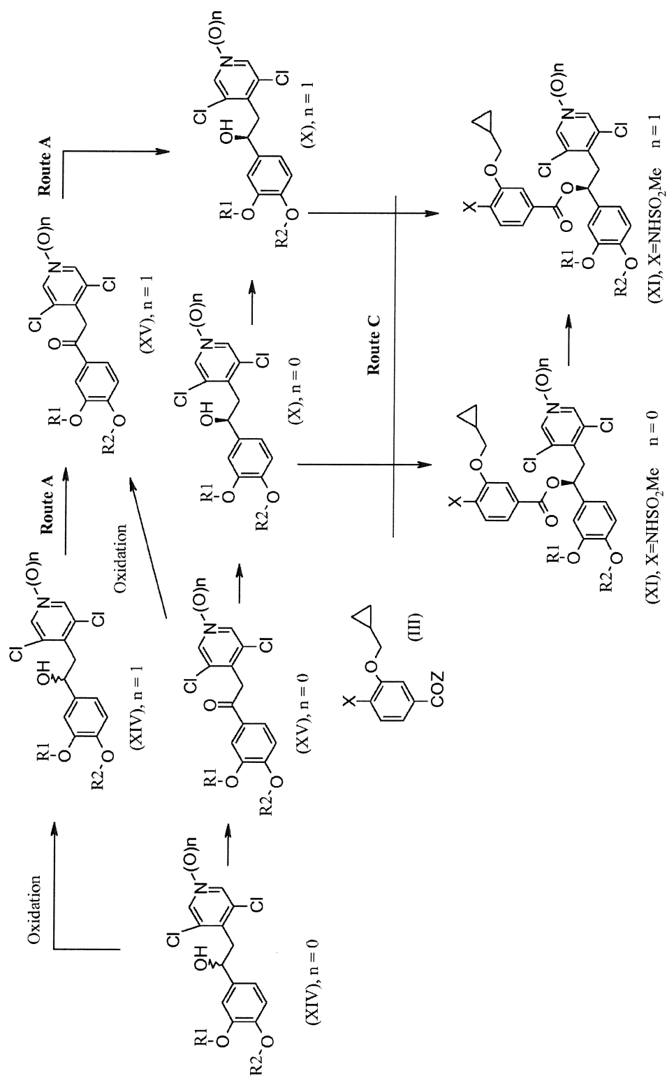
Scheme 5
