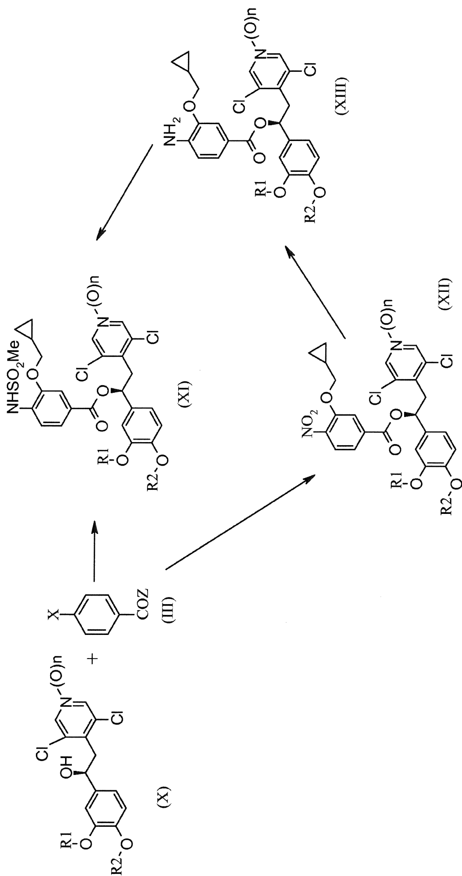
Scheme 6
