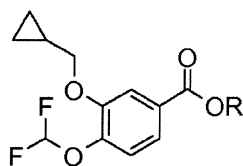
Intermediate B''
