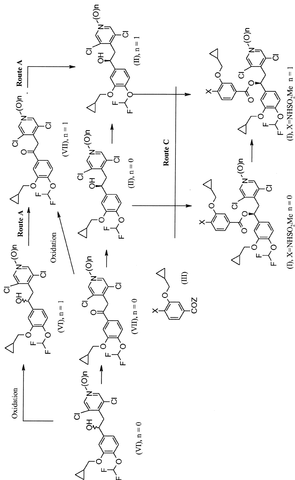
Scheme 2
