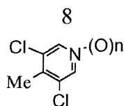
Intermediate D
