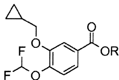
Intermediate B''
