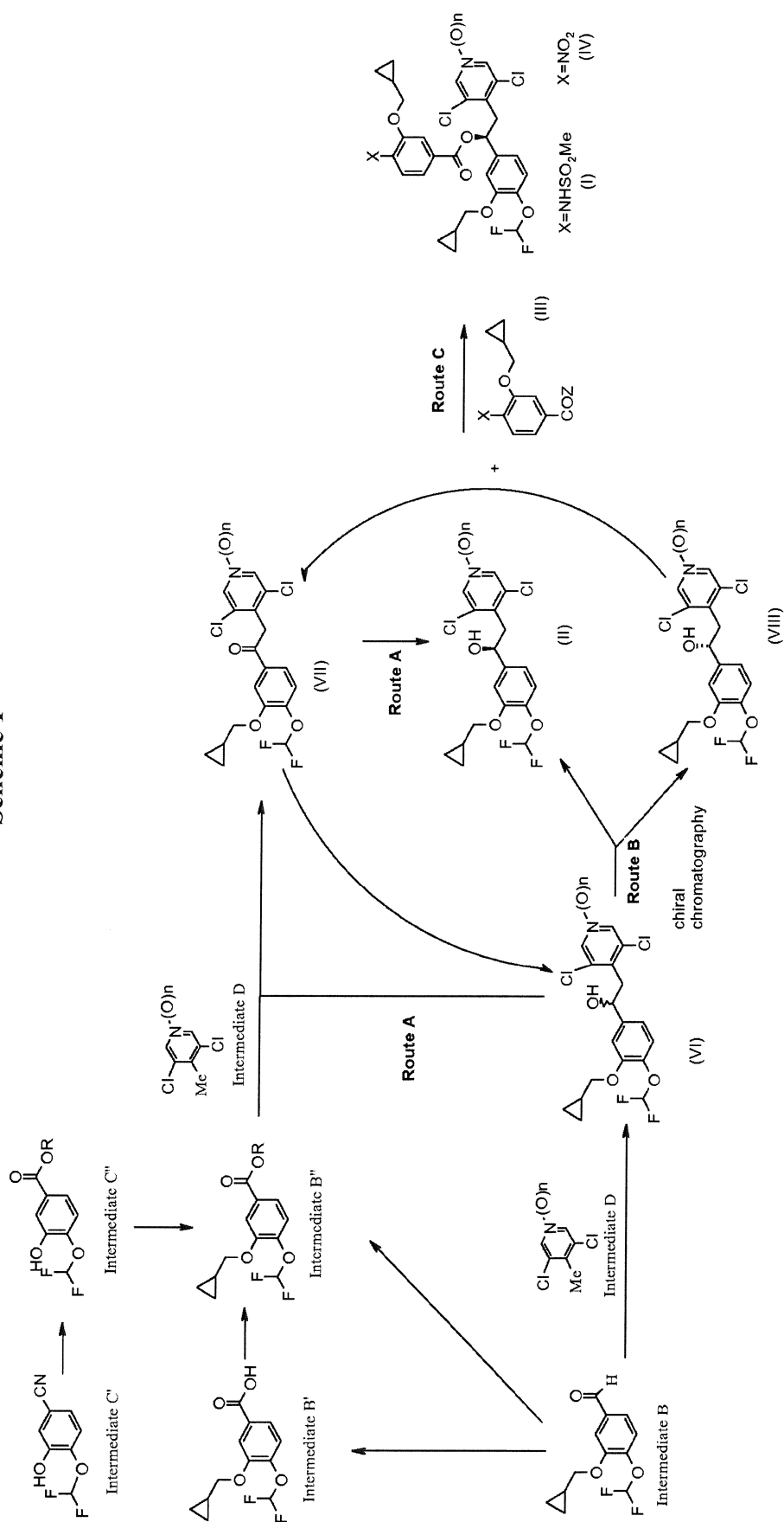
Scheme 1
