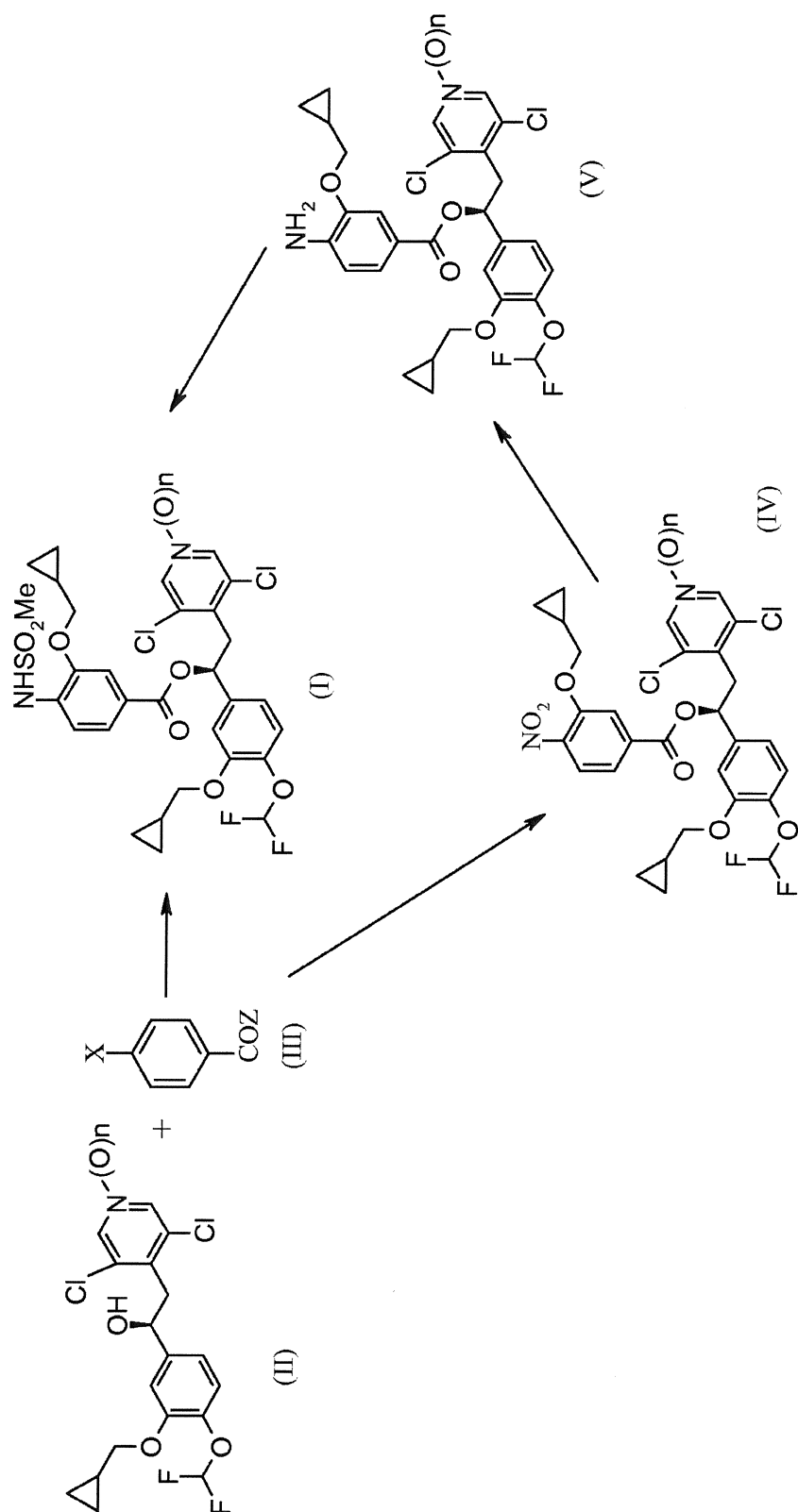
Scheme 3
