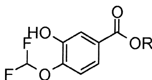
Intermediate C''
