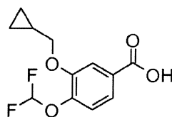
Intermediate B'
