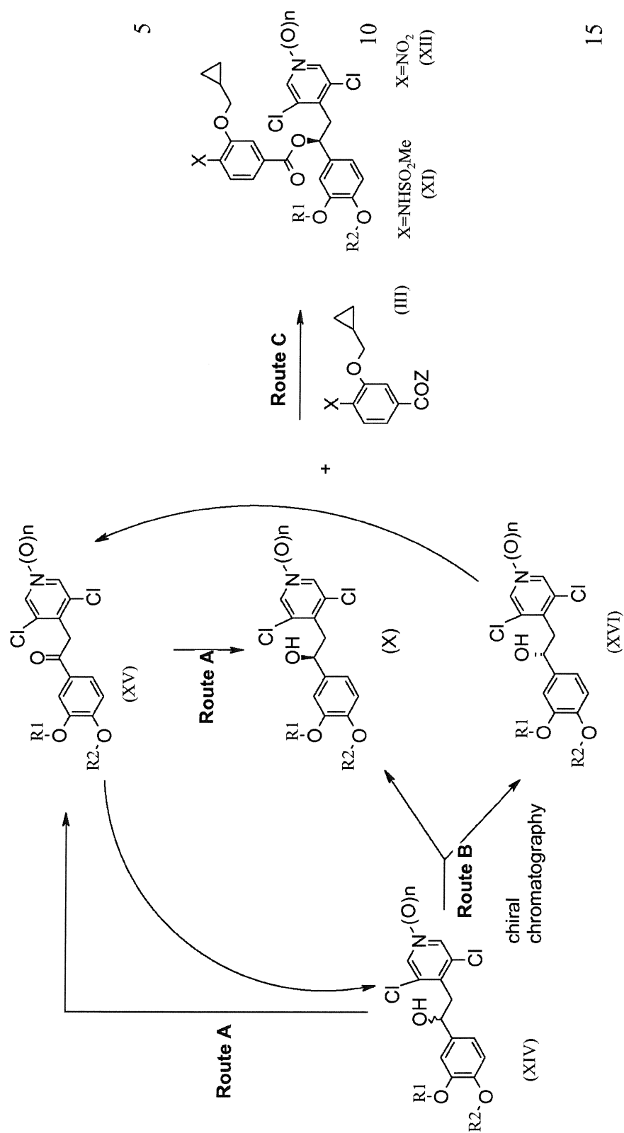
Scheme 4
