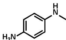
N-Methyl-p-phenylenediamine
