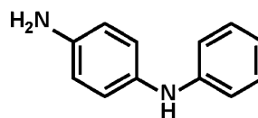
N-Phenyl-p-phenylenediamine
