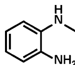
N-Methyl-1,2-phenylenediamine
