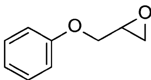
Phenyl glycidyl ether
