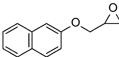
2-Naphthyl glycidyl ether
